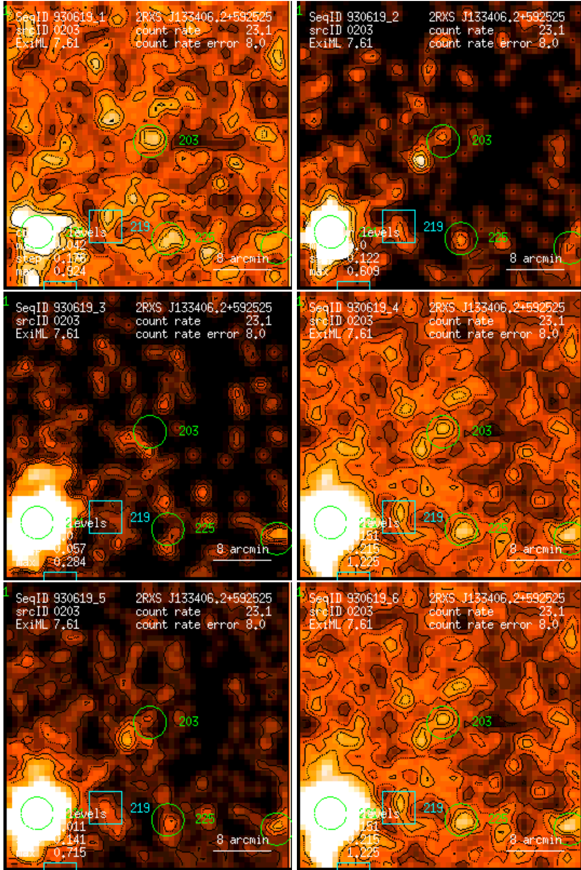
Figure 203: RASS 930619: detection 0203: band rate images, Gaussian filter: (1) PSPC channels 11 – 41, (2) 52 – 90, (3) 91 – 201, (4) 11 – 235, (5) 52 – 201, (6) 11 – 201. Broad band rates in counts/ks. Band rate contour levels in counts/ks/arcmin 2 .
