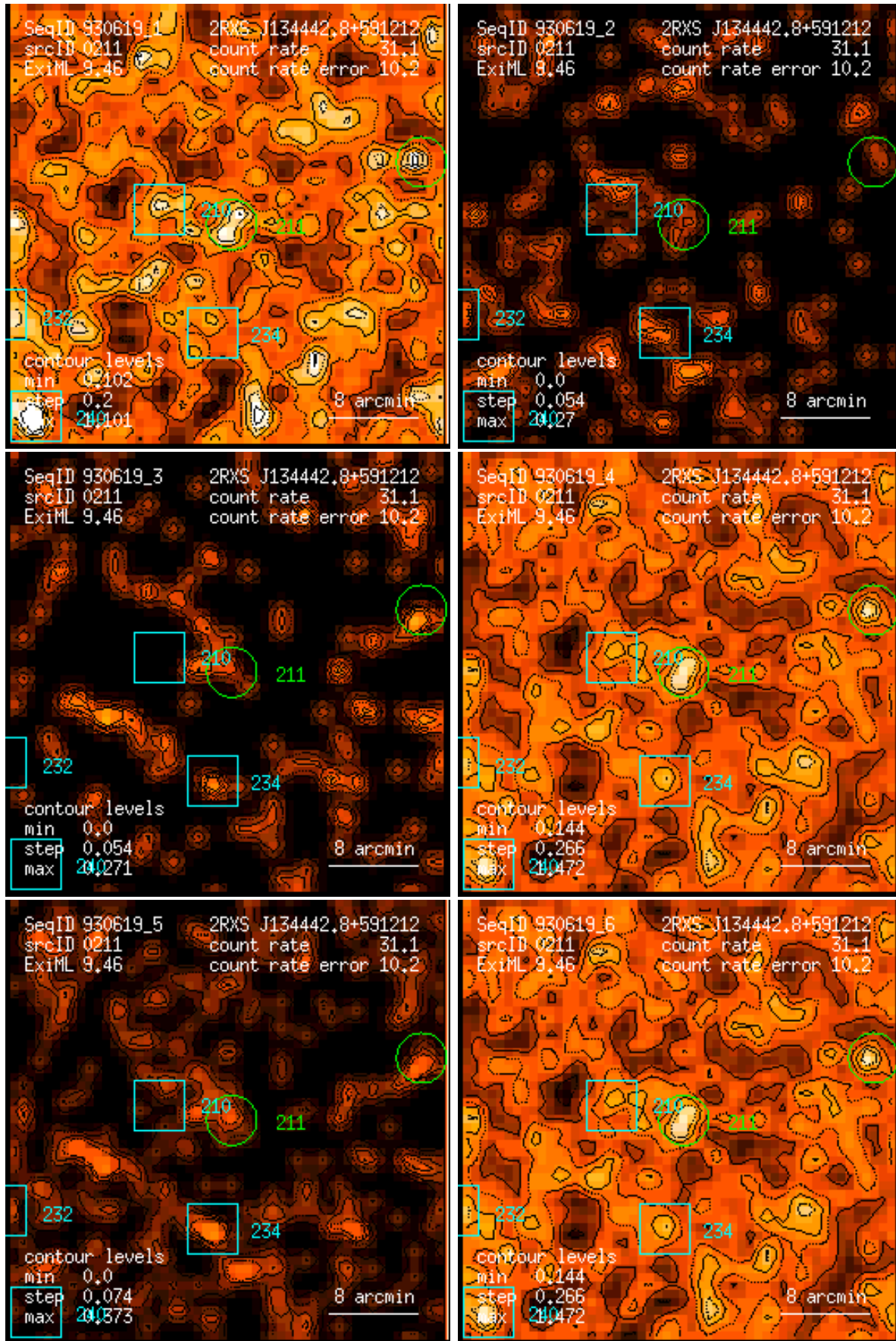
Figure 211: RASS 930619: detection 0211: band rate images, Gaussian filter: (1) PSPC channels 11 – 41, (2) 52 – 90, (3) 91 – 201, (4) 11 – 235, (5) 52 – 201, (6) 11 – 201. Broad band rates in counts/ks. Band rate contour levels in counts/ks/arcmin 2 .
