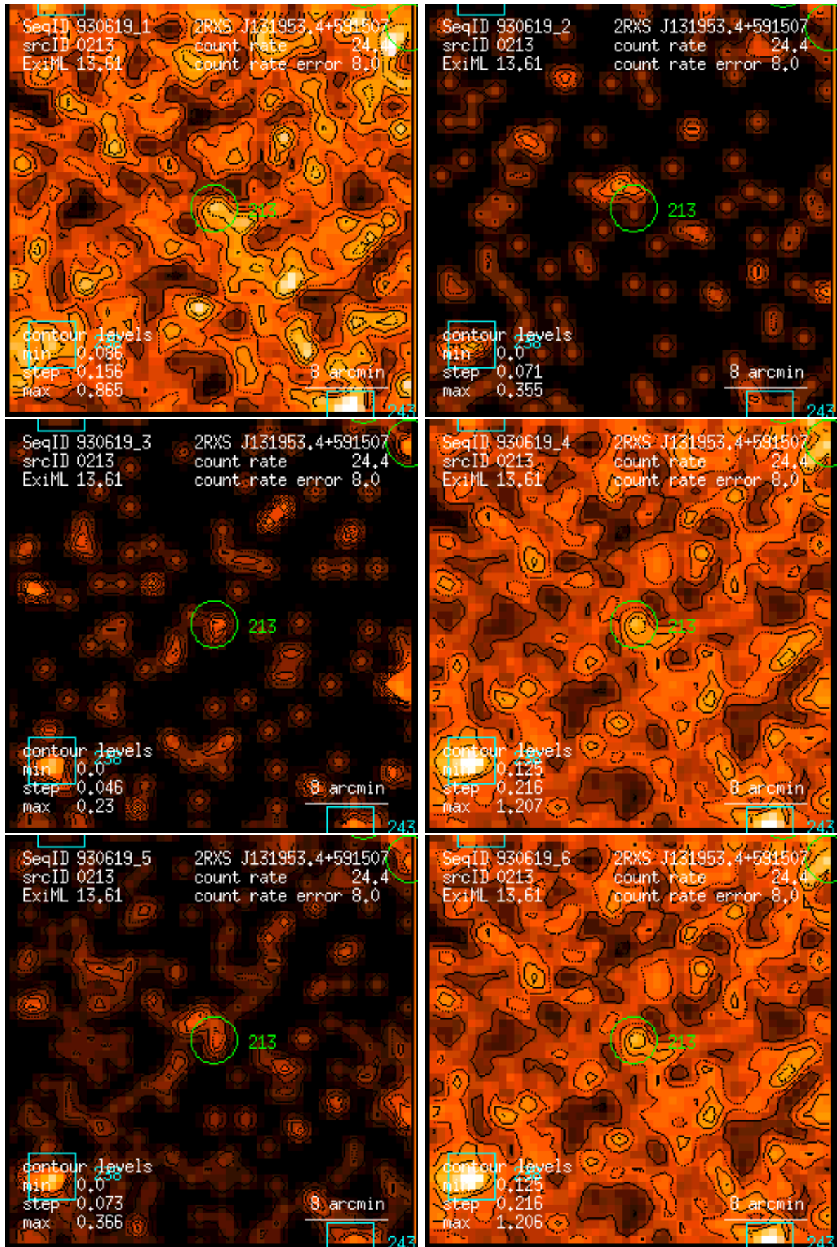
Figure 213: RASS 930619: detection 0213: band rate images, Gaussian filter: (1) PSPC channels 11 – 41, (2) 52 – 90, (3) 91 – 201, (4) 11 – 235, (5) 52 – 201, (6) 11 – 201. Broad band rates in counts/ks. Band rate contour levels in counts/ks/arcmin 2 .
