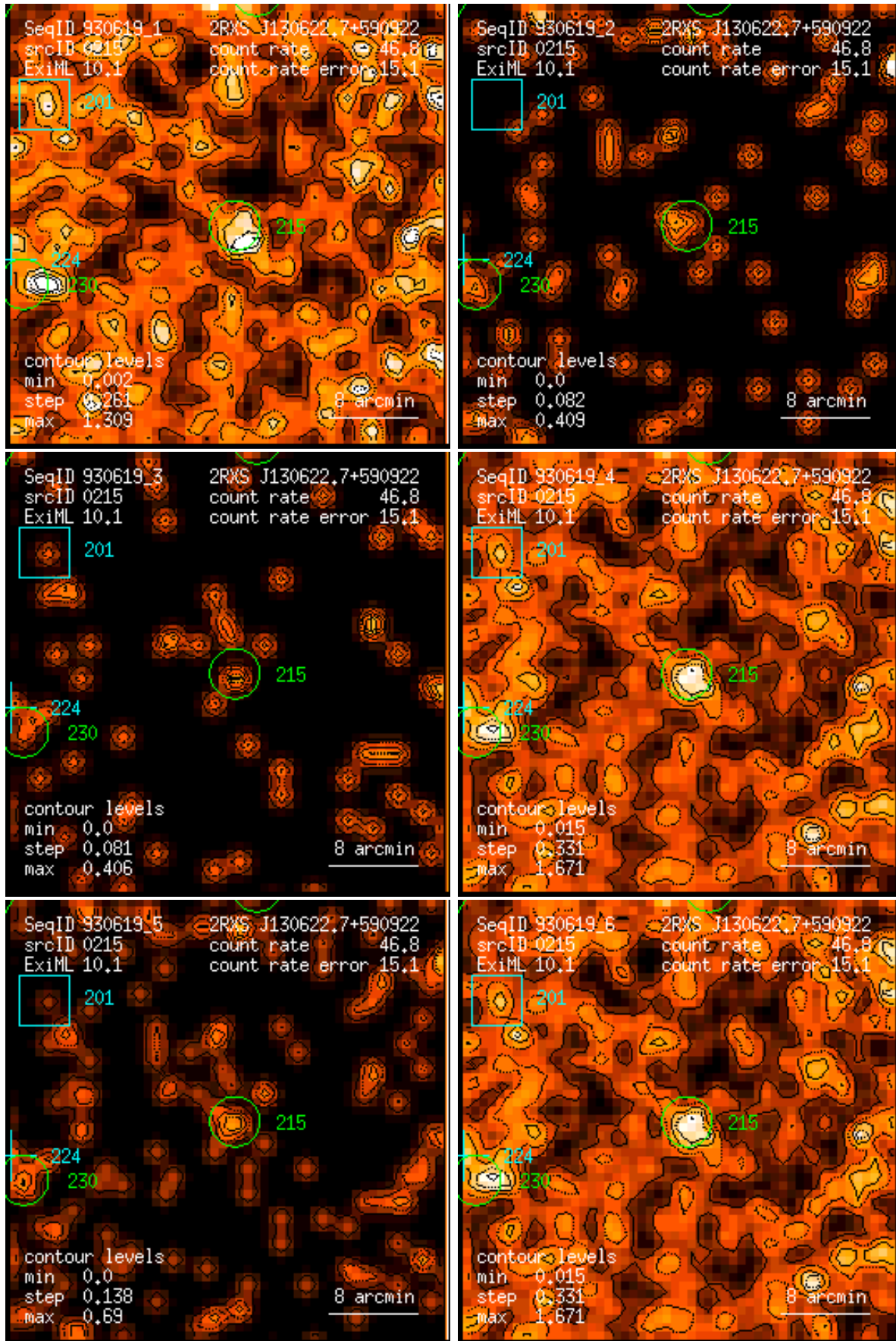
Figure 215: RASS 930619: detection 0215: band rate images, Gaussian filter: (1) PSPC channels 11 – 41, (2) 52 – 90, (3) 91 – 201, (4) 11 – 235, (5) 52 – 201, (6) 11 – 201. Broad band rates in counts/ks. Band rate contour levels in counts/ks/arcmin 2 .
