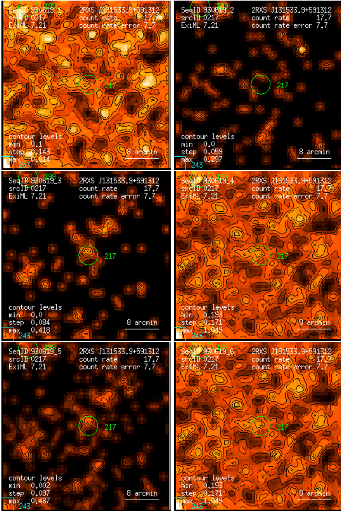
Figure 217: RASS 930619: detection 0217: band rate images, Gaussian filter: (1) PSPC channels 11 – 41, (2) 52 – 90, (3) 91 – 201, (4) 11 – 235, (5) 52 – 201, (6) 11 – 201. Broad band rates in counts/ks. Band rate contour levels in counts/ks/arcmin 2 .
