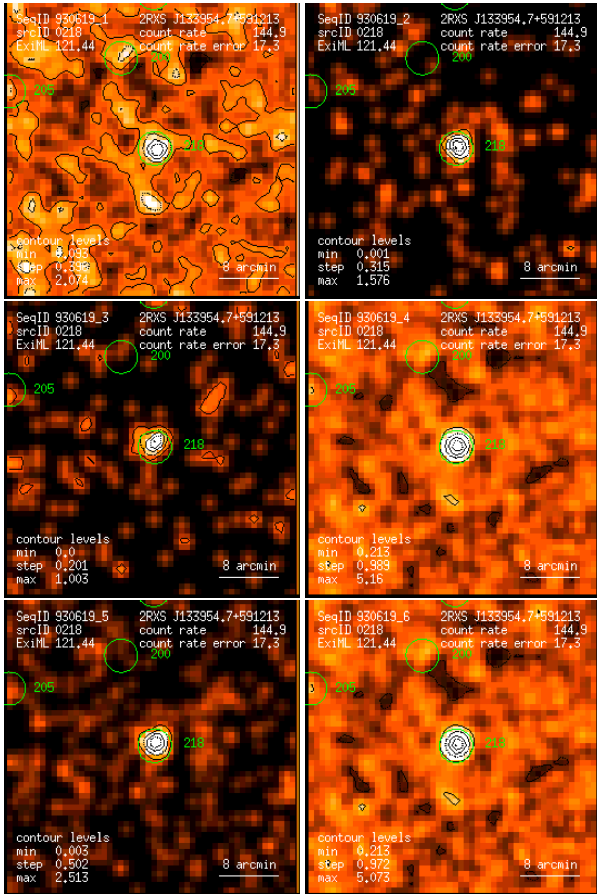
Figure 218: RASS 930619: detection 0218: band rate images, Gaussian filter: (1) PSPC channels 11 – 41, (2) 52 – 90, (3) 91 – 201, (4) 11 – 235, (5) 52 – 201, (6) 11 – 201. Broad band rates in counts/ks. Band rate contour levels in counts/ks/arcmin 2 .
