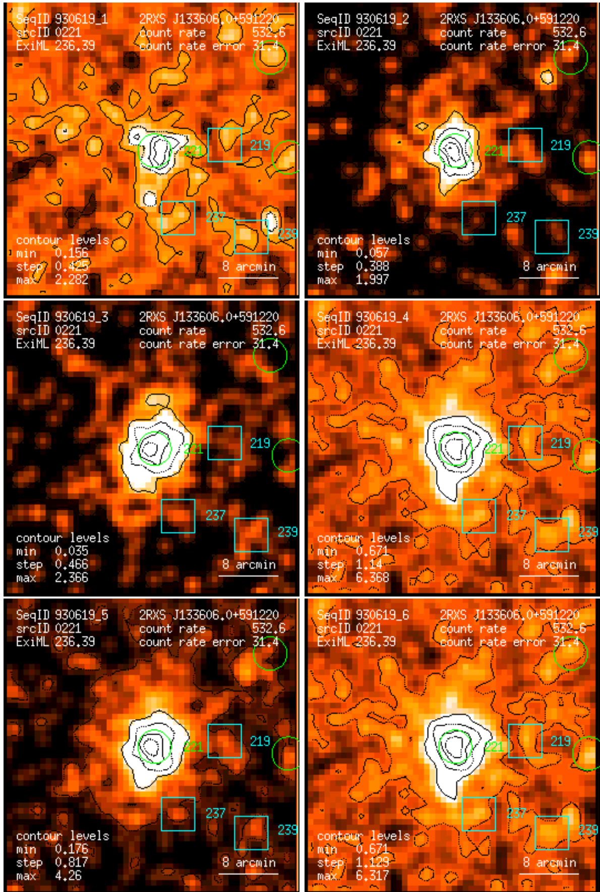
Figure 221: RASS 930619: detection 0221: band rate images, Gaussian filter: (1) PSPC channels 11 – 41, (2) 52 – 90, (3) 91 – 201, (4) 11 – 235, (5) 52 – 201, (6) 11 – 201. Broad band rates in counts/ks. Band rate contour levels in counts/ks/arcmin 2 .
