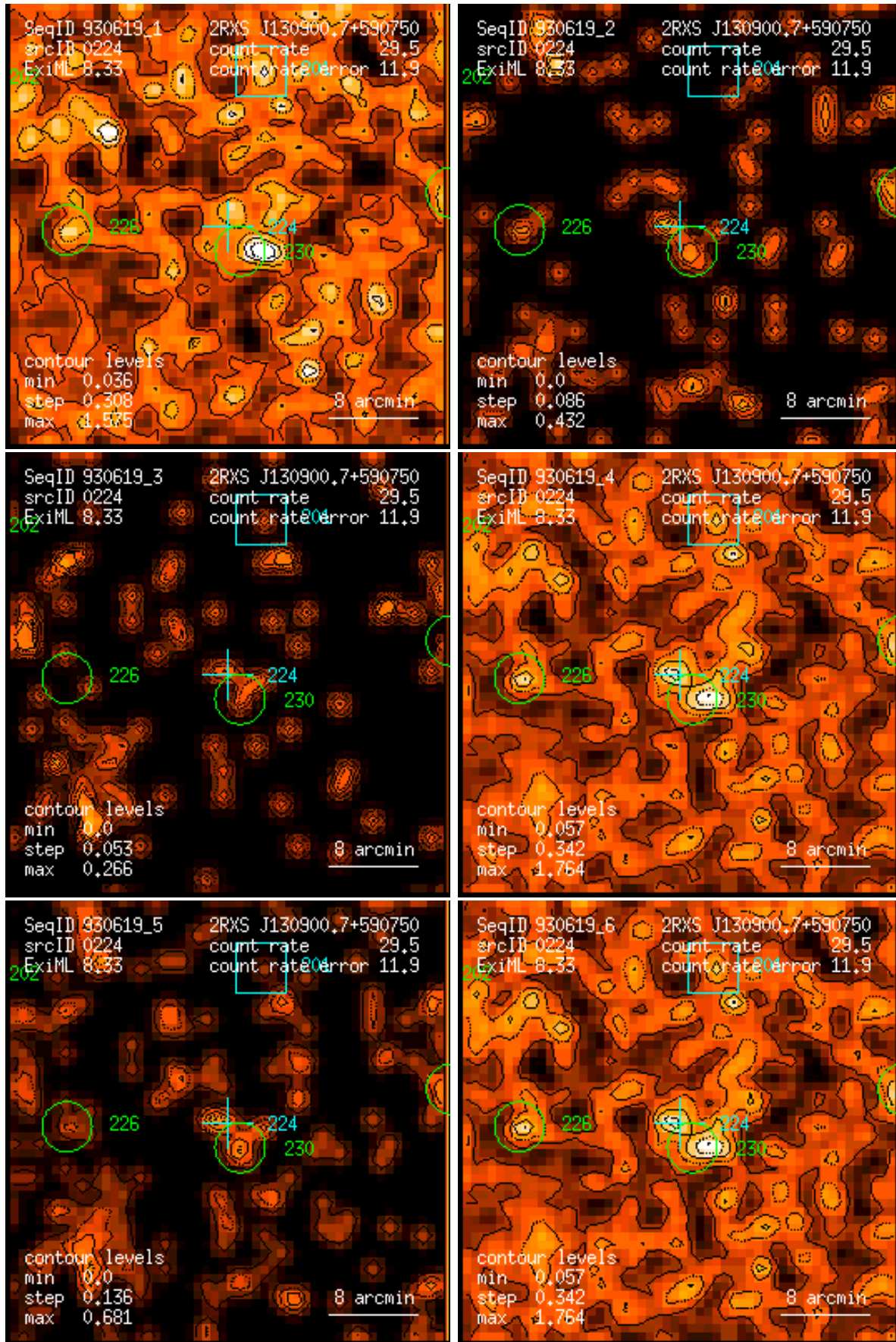
Figure 224: RASS 930619: detection 0224: band rate images, Gaussian filter: (1) PSPC channels 11 – 41, (2) 52 – 90, (3) 91 – 201, (4) 11 – 235, (5) 52 – 201, (6) 11 – 201. Broad band rates in counts/ks. Band rate contour levels in counts/ks/arcmin 2 .
