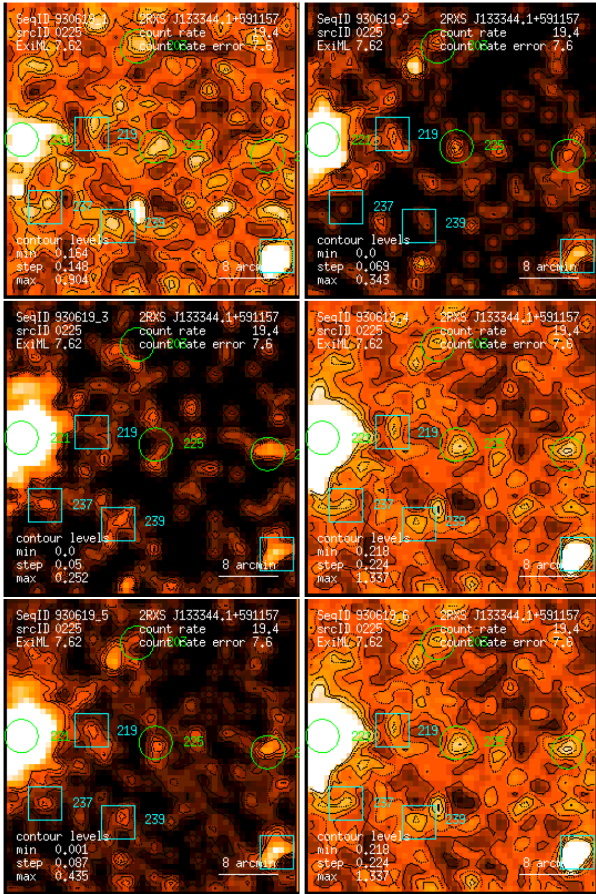
Figure 225: RASS 930619: detection 0225: band rate images, Gaussian filter: (1) PSPC channels 11 – 41, (2) 52 – 90, (3) 91 – 201, (4) 11 – 235, (5) 52 – 201, (6) 11 – 201. Broad band rates in counts/ks. Band rate contour levels in counts/ks/arcmin 2 .
