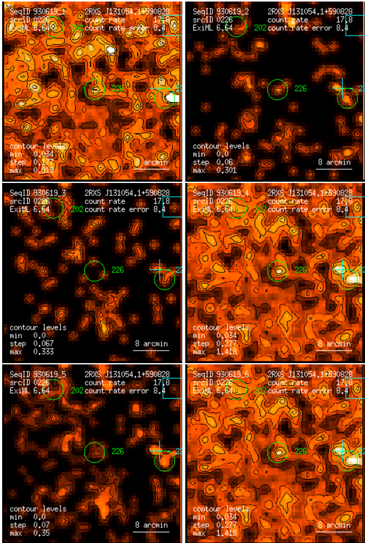
Figure 226: RASS 930619: detection 0226: band rate images, Gaussian filter: (1) PSPC channels 11 – 41, (2) 52 – 90, (3) 91 – 201, (4) 11 – 235, (5) 52 – 201, (6) 11 – 201. Broad band rates in counts/ks. Band rate contour levels in counts/ks/arcmin 2 .
