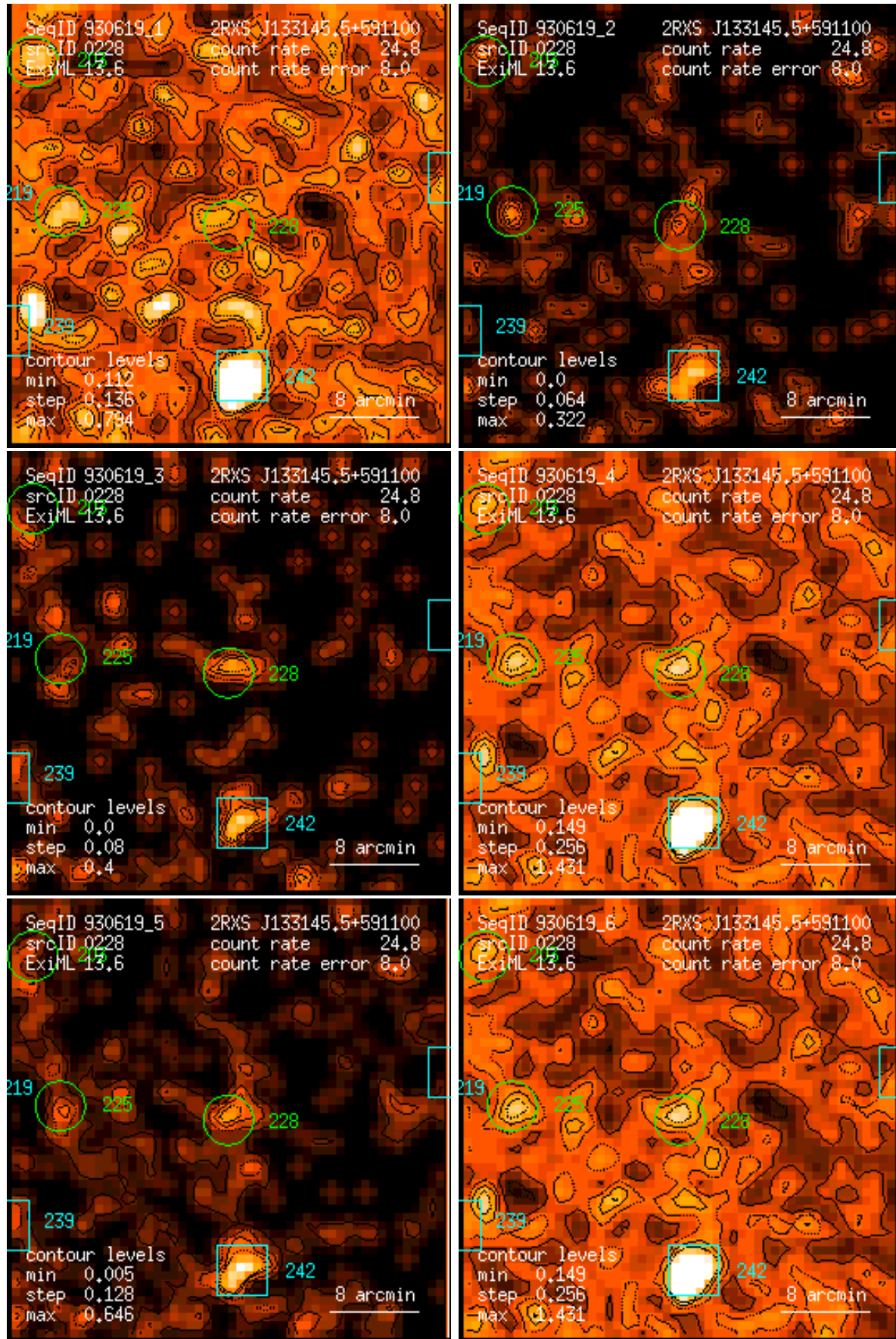
Figure 228: RASS 930619: detection 0228: band rate images, Gaussian filter: (1) PSPC channels 11 – 41, (2) 52 – 90, (3) 91 – 201, (4) 11 – 235, (5) 52 – 201, (6) 11 – 201. Broad band rates in counts/ks. Band rate contour levels in counts/ks/arcmin 2 .
