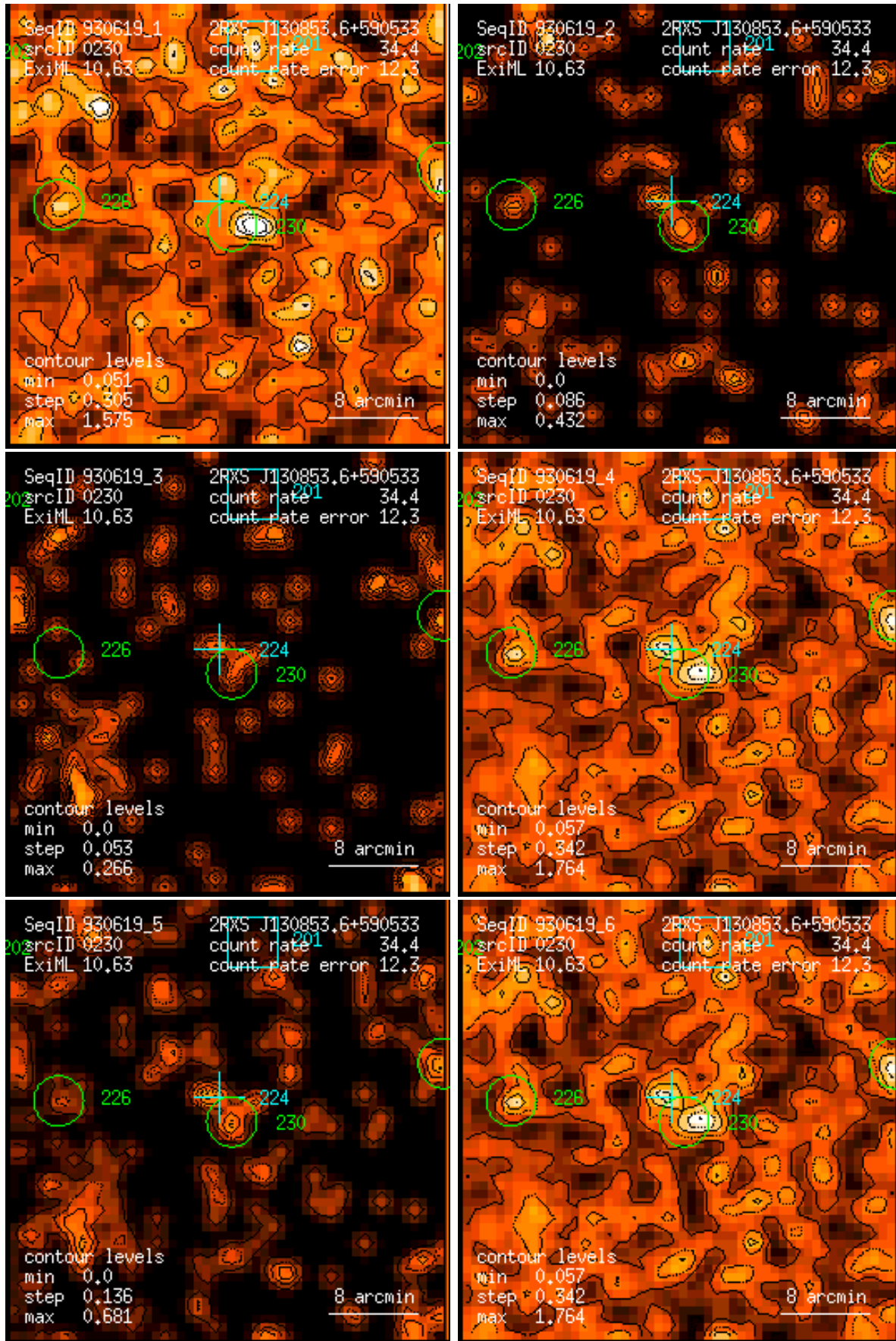
Figure 230: RASS 930619: detection 0230: band rate images, Gaussian filter: (1) PSPC channels 11 – 41, (2) 52 – 90, (3) 91 – 201, (4) 11 – 235, (5) 52 – 201, (6) 11 – 201. Broad band rates in counts/ks. Band rate contour levels in counts/ks/arcmin 2 .
