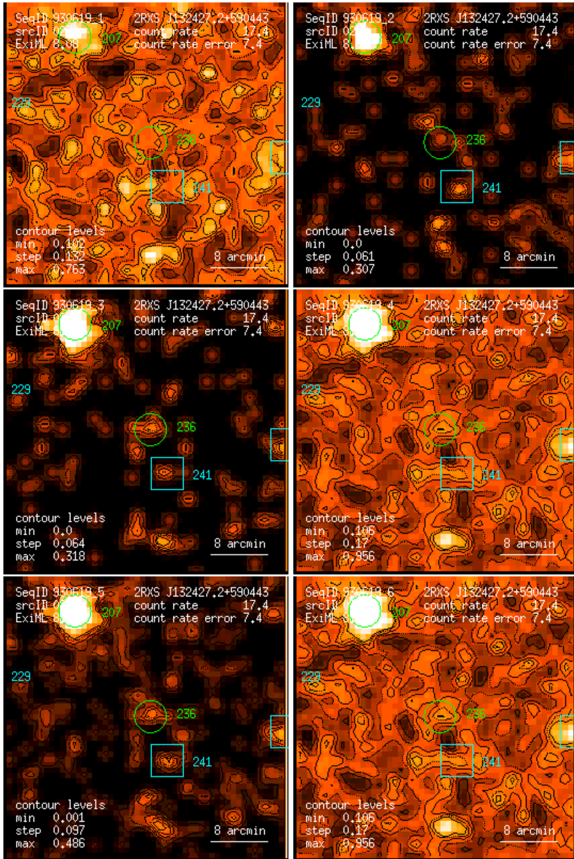
Figure 236: RASS 930619: detection 0236: band rate images, Gaussian filter: (1) PSPC channels 11 – 41, (2) 52 – 90, (3) 91 – 201, (4) 11 – 235, (5) 52 – 201, (6) 11 – 201. Broad band rates in counts/ks. Band rate contour levels in counts/ks/arcmin 2 .
