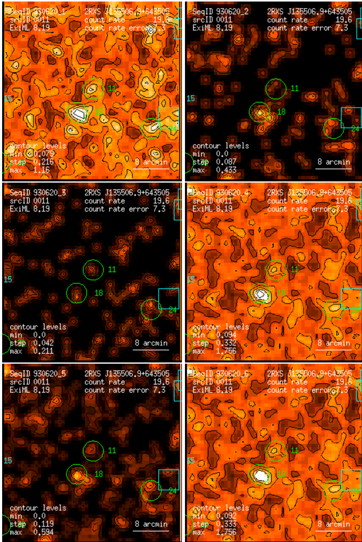
Figure 11: RASS 930620: detection 0011: band rate images, Gaussian filter: (1) PSPC channels 11 – 41, (2) 52 – 90, (3) 91 – 201, (4) 11 – 235, (5) 52 – 201, (6) 11 – 201. Broad band rates in counts/ks. Band rate contour levels in counts/ks/arcmin 2 .
