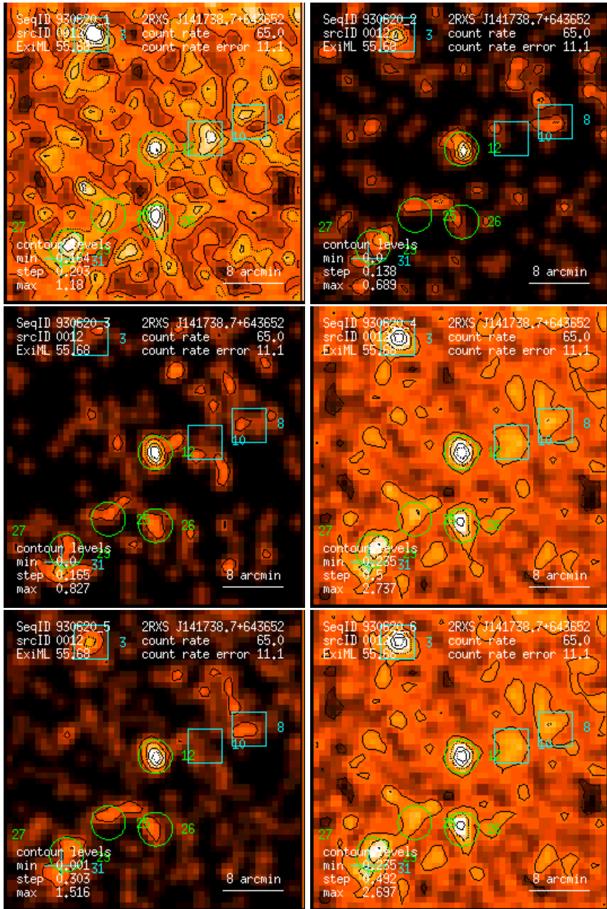
Figure 12: RASS 930620: detection 0012: band rate images, Gaussian filter: (1) PSPC channels 11 – 41, (2) 52 – 90, (3) 91 – 201, (4) 11 – 235, (5) 52 – 201, (6) 11 – 201. Broad band rates in counts/ks. Band rate contour levels in counts/ks/arcmin 2 .
