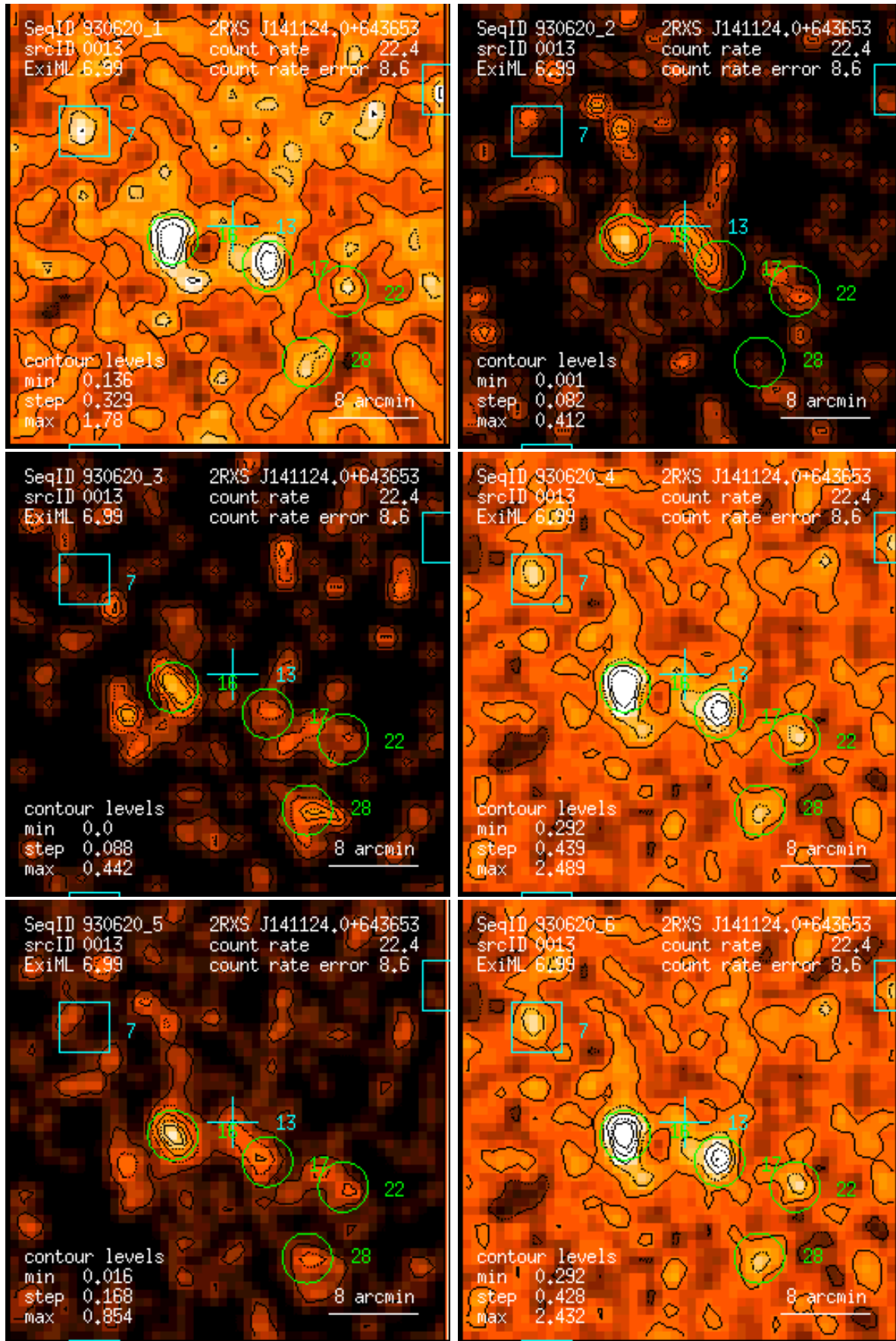
Figure 13: RASS 930620: detection 0013: band rate images, Gaussian filter: (1) PSPC channels 11 – 41, (2) 52 – 90, (3) 91 – 201, (4) 11 – 235, (5) 52 – 201, (6) 11 – 201. Broad band rates in counts/ks. Band rate contour levels in counts/ks/arcmin 2 .
