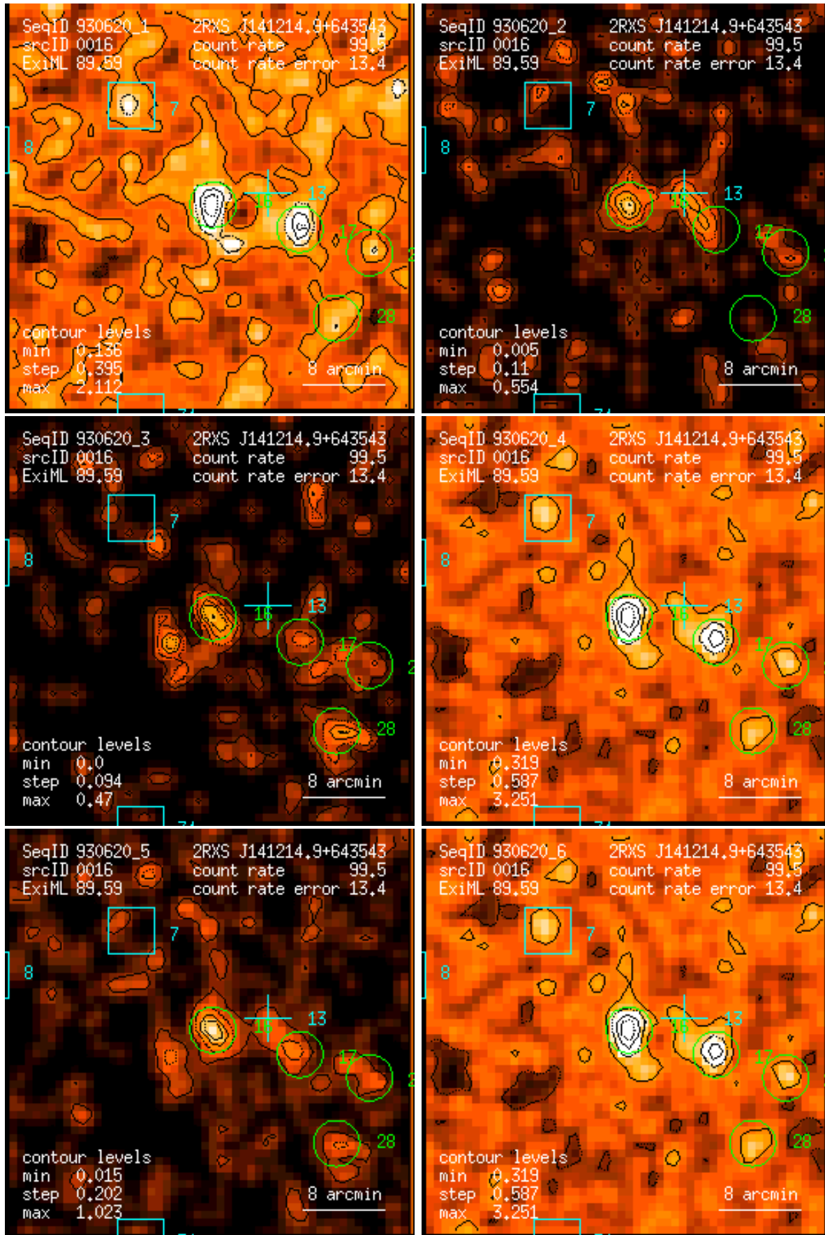
Figure 16: RASS 930620: detection 0016: band rate images, Gaussian filter: (1) PSPC channels 11 – 41, (2) 52 – 90, (3) 91 – 201, (4) 11 – 235, (5) 52 – 201, (6) 11 – 201. Broad band rates in counts/ks. Band rate contour levels in counts/ks/arcmin 2 .
