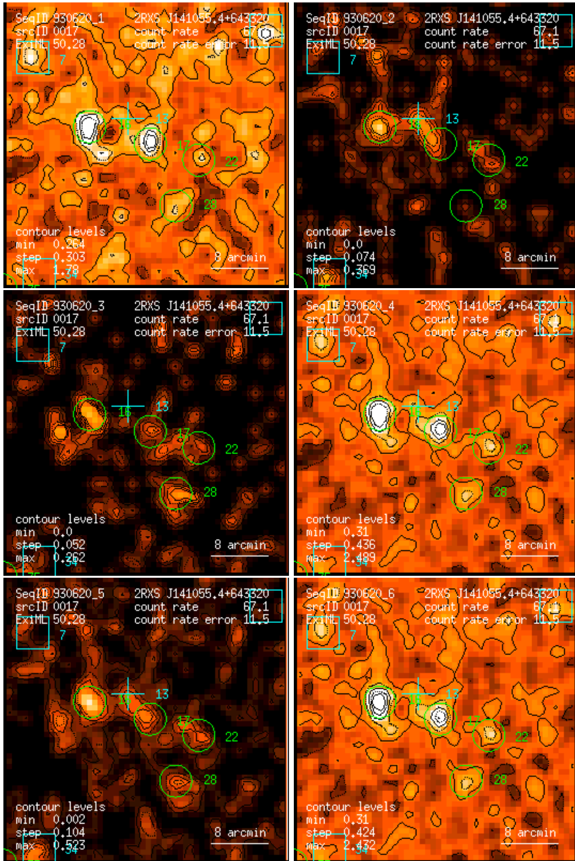
Figure 17: RASS 930620: detection 0017: band rate images, Gaussian filter: (1) PSPC channels 11 – 41, (2) 52 – 90, (3) 91 – 201, (4) 11 – 235, (5) 52 – 201, (6) 11 – 201. Broad band rates in counts/ks. Band rate contour levels in counts/ks/arcmin 2 .
