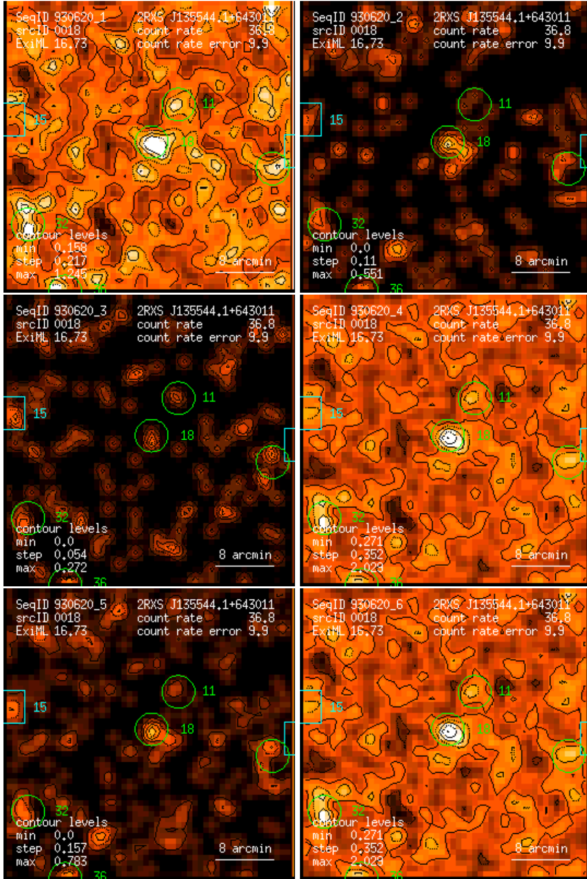
Figure 18: RASS 930620: detection 0018: band rate images, Gaussian filter: (1) PSPC channels 11 – 41, (2) 52 – 90, (3) 91 – 201, (4) 11 – 235, (5) 52 – 201, (6) 11 – 201. Broad band rates in counts/ks. Band rate contour levels in counts/ks/arcmin 2 .
