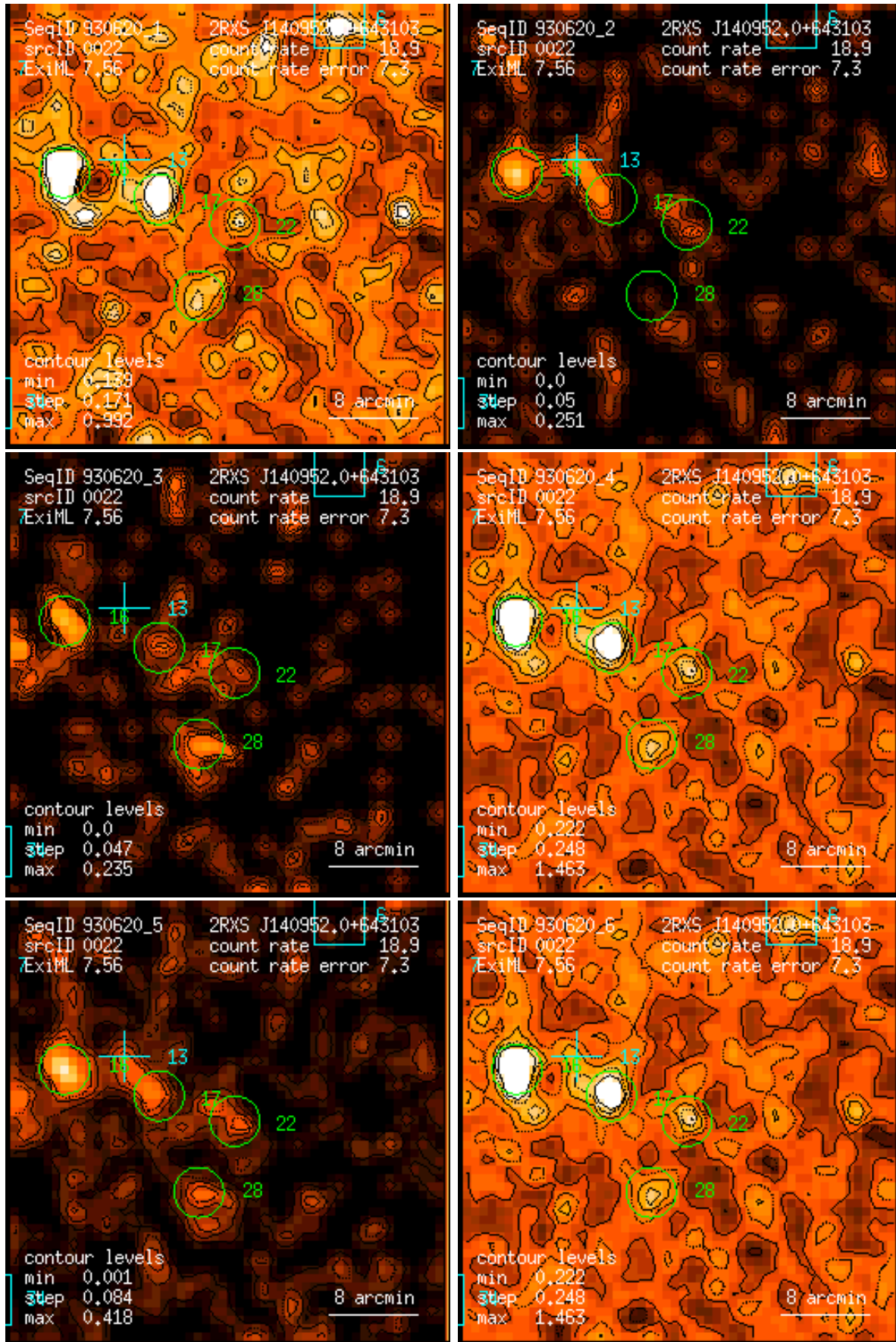
Figure 22: RASS 930620: detection 0022: band rate images, Gaussian filter: (1) PSPC channels 11 – 41, (2) 52 – 90, (3) 91 – 201, (4) 11 – 235, (5) 52 – 201, (6) 11 – 201. Broad band rates in counts/ks. Band rate contour levels in counts/ks/arcmin 2 .
