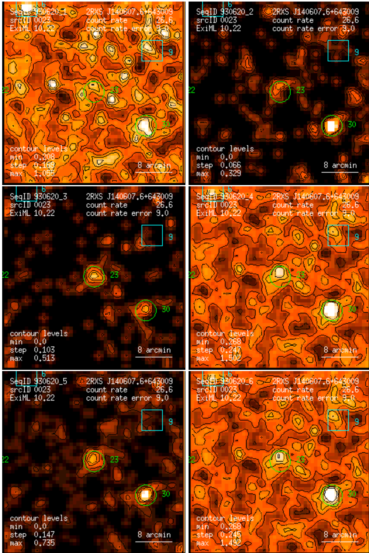
Figure 23: RASS 930620: detection 0023: band rate images, Gaussian filter: (1) PSPC channels 11 – 41, (2) 52 – 90, (3) 91 – 201, (4) 11 – 235, (5) 52 – 201, (6) 11 – 201. Broad band rates in counts/ks. Band rate contour levels in counts/ks/arcmin 2 .
