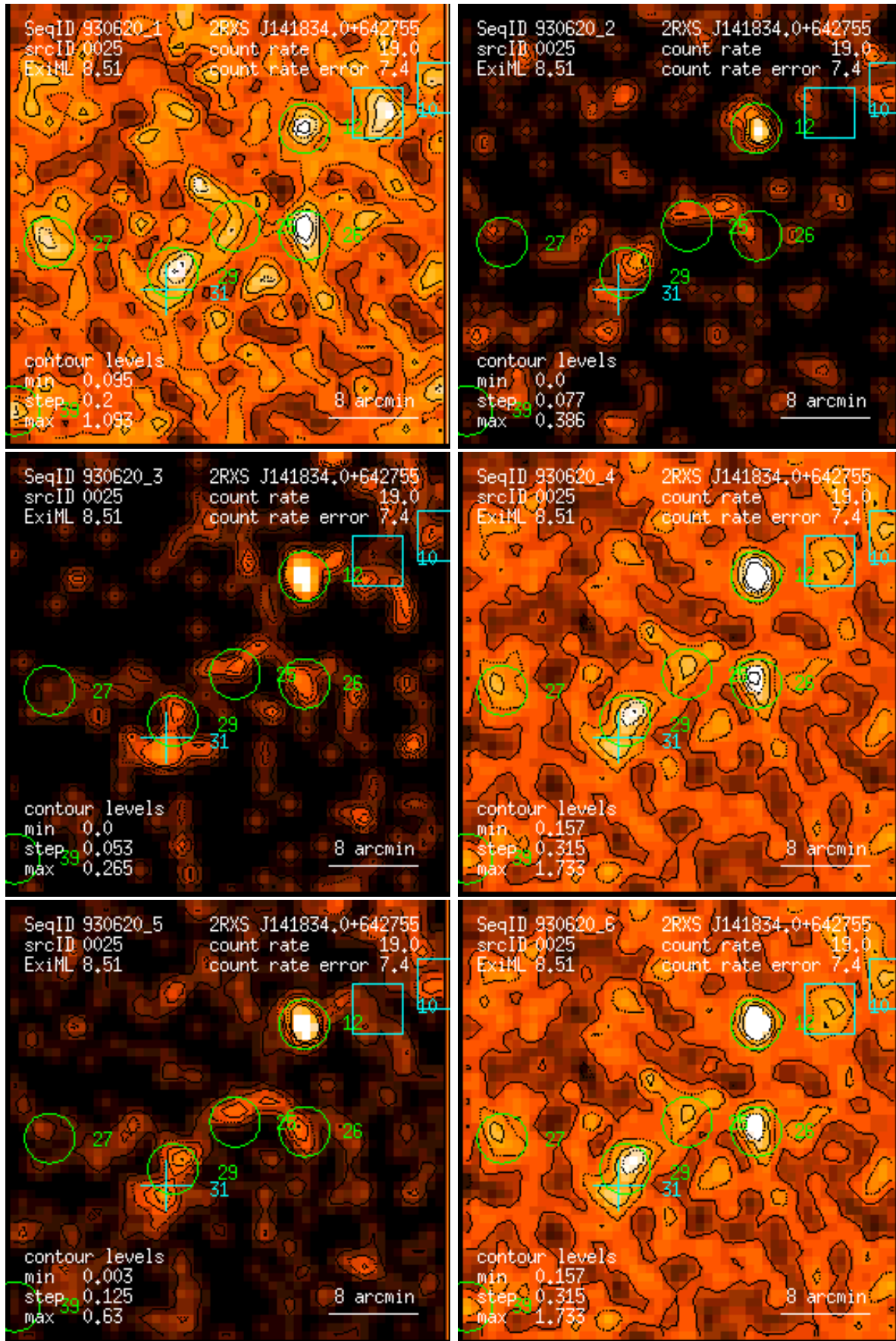
Figure 25: RASS 930620: detection 0025: band rate images, Gaussian filter: (1) PSPC channels 11 – 41, (2) 52 – 90, (3) 91 – 201, (4) 11 – 235, (5) 52 – 201, (6) 11 – 201. Broad band rates in counts/ks. Band rate contour levels in counts/ks/arcmin 2 .
