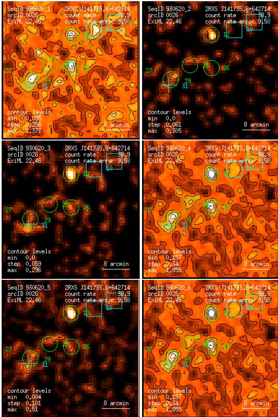
Figure 26: RASS 930620: detection 0026: band rate images, Gaussian filter: (1) PSPC channels 11 – 41, (2) 52 – 90, (3) 91 – 201, (4) 11 – 235, (5) 52 – 201, (6) 11 – 201. Broad band rates in counts/ks. Band rate contour levels in counts/ks/arcmin 2 .
