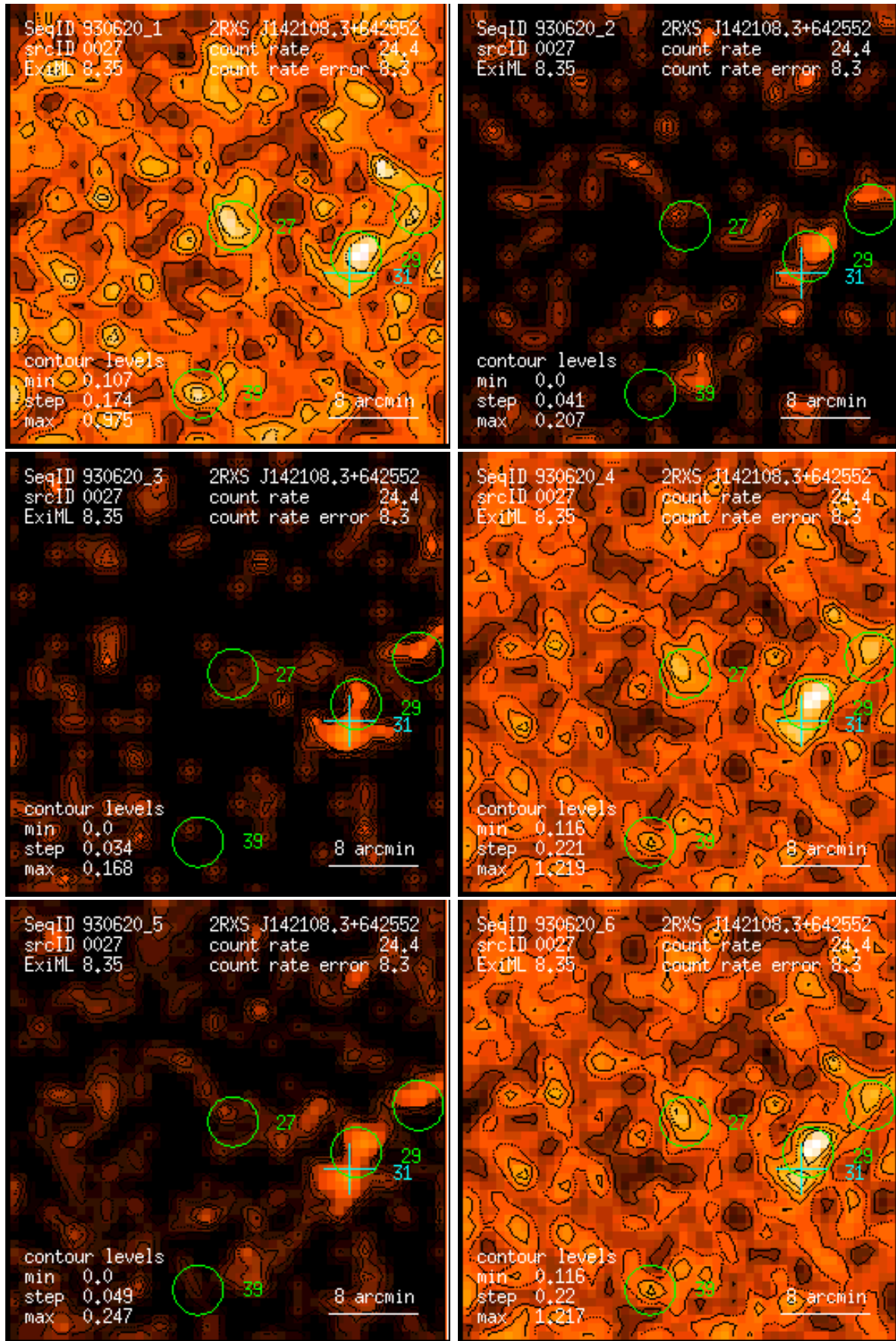
Figure 27: RASS 930620: detection 0027: band rate images, Gaussian filter: (1) PSPC channels 11 – 41, (2) 52 – 90, (3) 91 – 201, (4) 11 – 235, (5) 52 – 201, (6) 11 – 201. Broad band rates in counts/ks. Band rate contour levels in counts/ks/arcmin 2 .
