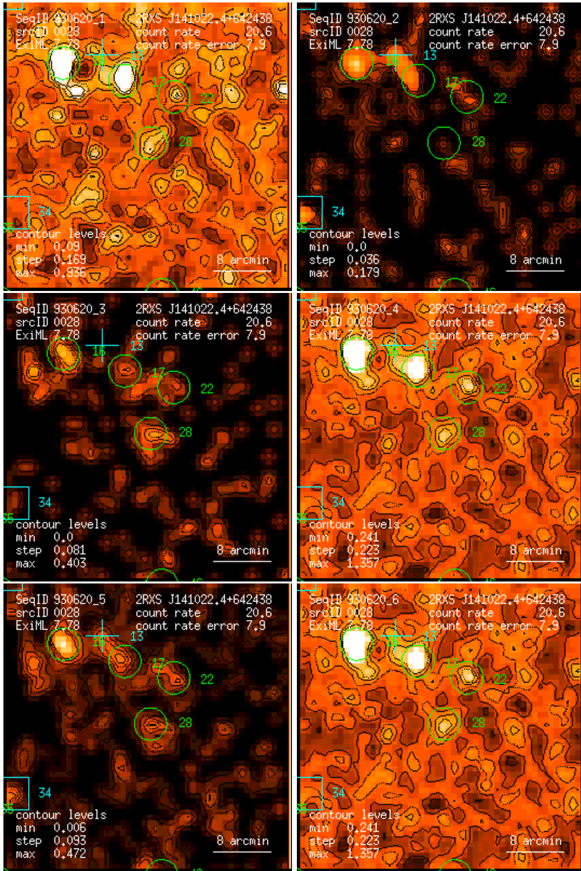
Figure 28: RASS 930620: detection 0028: band rate images, Gaussian filter: (1) PSPC channels 11 – 41, (2) 52 – 90, (3) 91 – 201, (4) 11 – 235, (5) 52 – 201, (6) 11 – 201. Broad band rates in counts/ks. Band rate contour levels in counts/ks/arcmin 2 .
