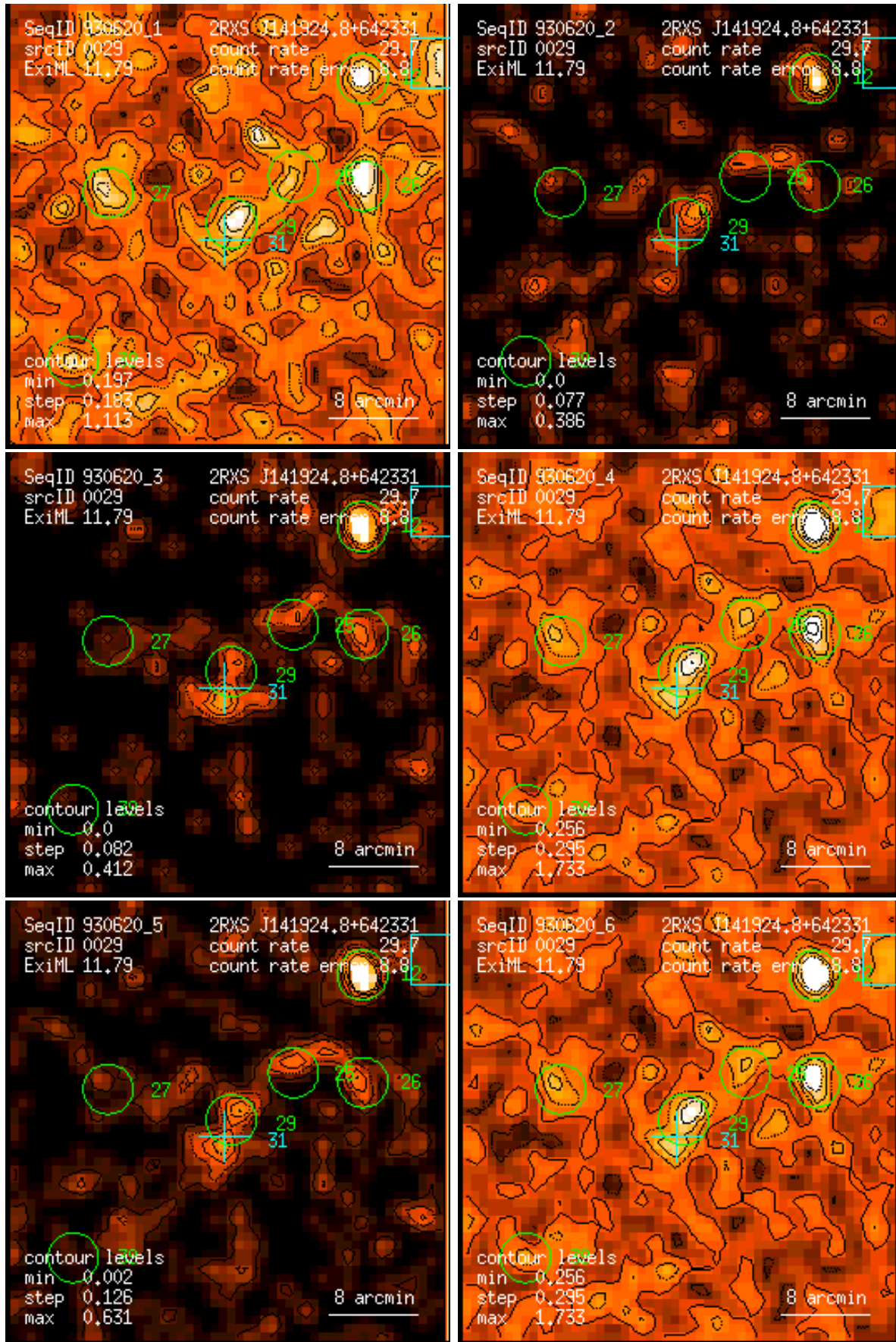
Figure 29: RASS 930620: detection 0029: band rate images, Gaussian filter: (1) PSPC channels 11 – 41, (2) 52 – 90, (3) 91 – 201, (4) 11 – 235, (5) 52 – 201, (6) 11 – 201. Broad band rates in counts/ks. Band rate contour levels in counts/ks/arcmin 2 .
