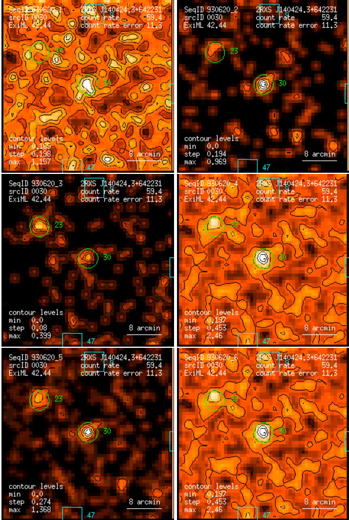
Figure 30: RASS 930620: detection 0030: band rate images, Gaussian filter: (1) PSPC channels 11 – 41, (2) 52 – 90, (3) 91 – 201, (4) 11 – 235, (5) 52 – 201, (6) 11 – 201. Broad band rates in counts/ks. Band rate contour levels in counts/ks/arcmin 2 .
