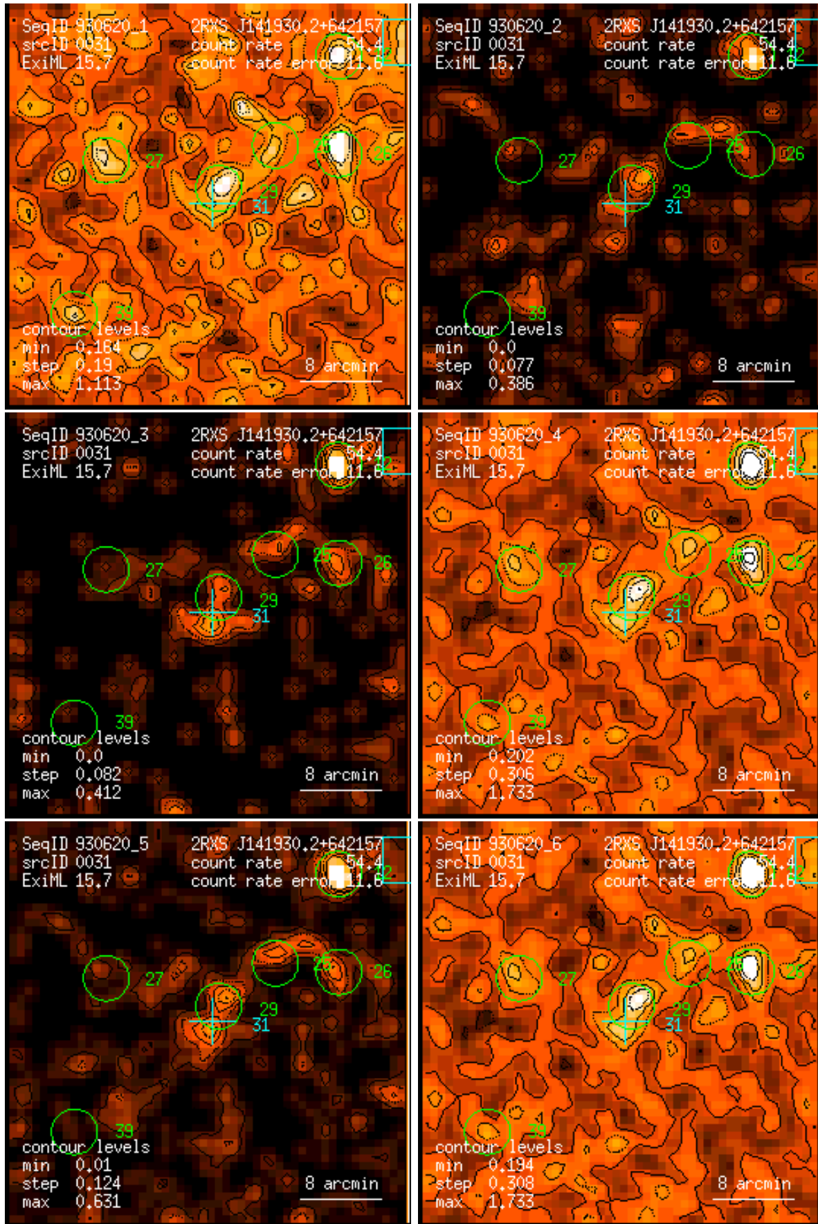
Figure 31: RASS 930620: detection 0031: band rate images, Gaussian filter: (1) PSPC channels 11 – 41, (2) 52 – 90, (3) 91 – 201, (4) 11 – 235, (5) 52 – 201, (6) 11 – 201. Broad band rates in counts/ks. Band rate contour levels in counts/ks/arcmin 2 .
