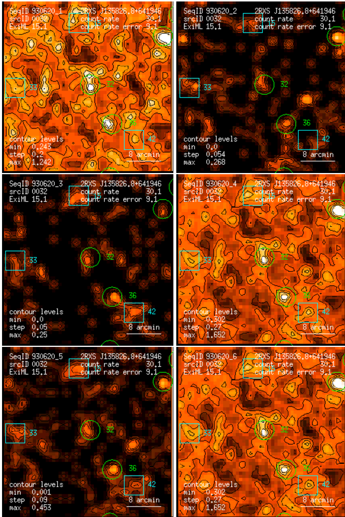
Figure 32: RASS 930620: detection 0032: band rate images, Gaussian filter: (1) PSPC channels 11 – 41, (2) 52 – 90, (3) 91 – 201, (4) 11 – 235, (5) 52 – 201, (6) 11 – 201. Broad band rates in counts/ks. Band rate contour levels in counts/ks/arcmin 2 .
