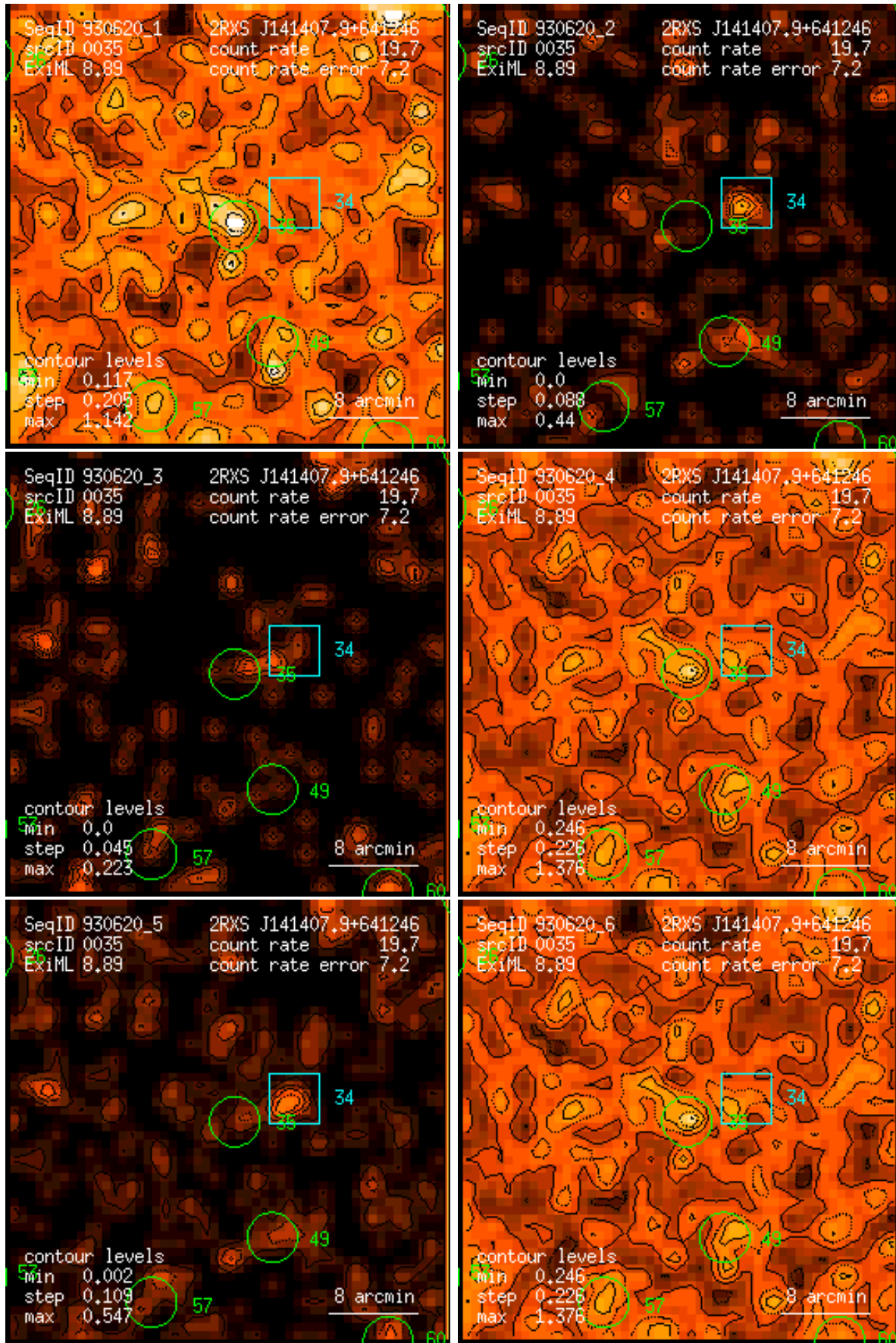
Figure 35: RASS 930620: detection 0035: band rate images, Gaussian filter: (1) PSPC channels 11 – 41, (2) 52 – 90, (3) 91 – 201, (4) 11 – 235, (5) 52 – 201, (6) 11 – 201. Broad band rates in counts/ks. Band rate contour levels in counts/ks/arcmin 2 .
