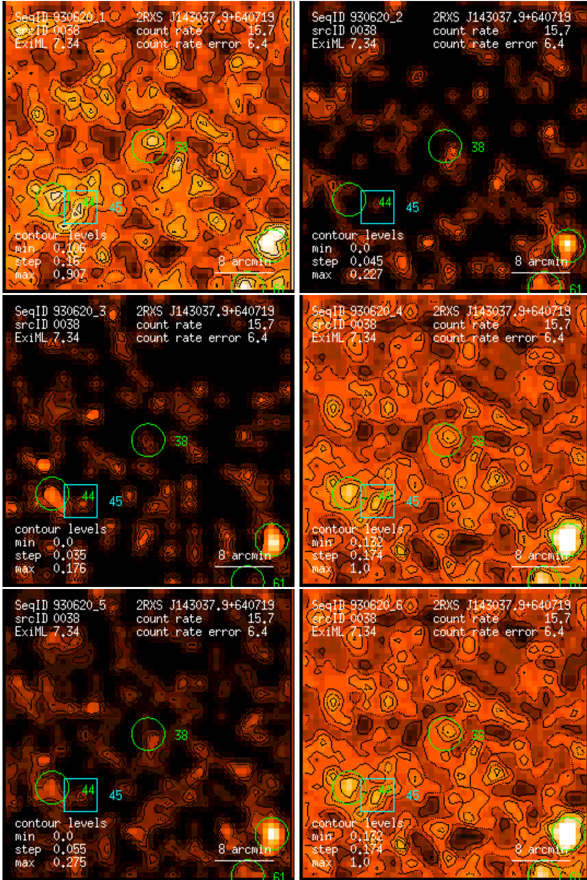
Figure 38: RASS 930620: detection 0038: band rate images, Gaussian filter: (1) PSPC channels 11 – 41, (2) 52 – 90, (3) 91 – 201, (4) 11 – 235, (5) 52 – 201, (6) 11 – 201. Broad band rates in counts/ks. Band rate contour levels in counts/ks/arcmin 2 .
