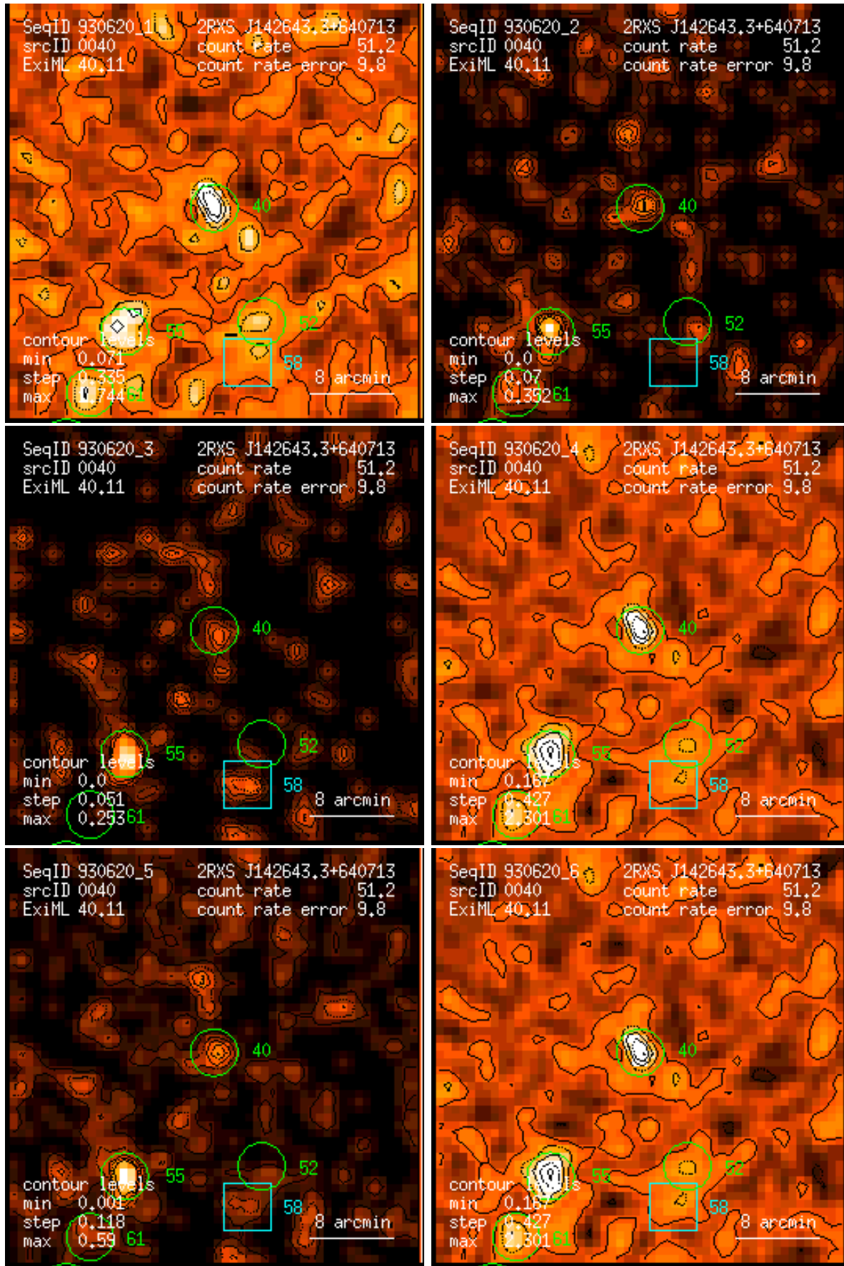
Figure 40: RASS 930620: detection 0040: band rate images, Gaussian filter: (1) PSPC channels 11 – 41, (2) 52 – 90, (3) 91 – 201, (4) 11 – 235, (5) 52 – 201, (6) 11 – 201. Broad band rates in counts/ks. Band rate contour levels in counts/ks/arcmin 2 .
