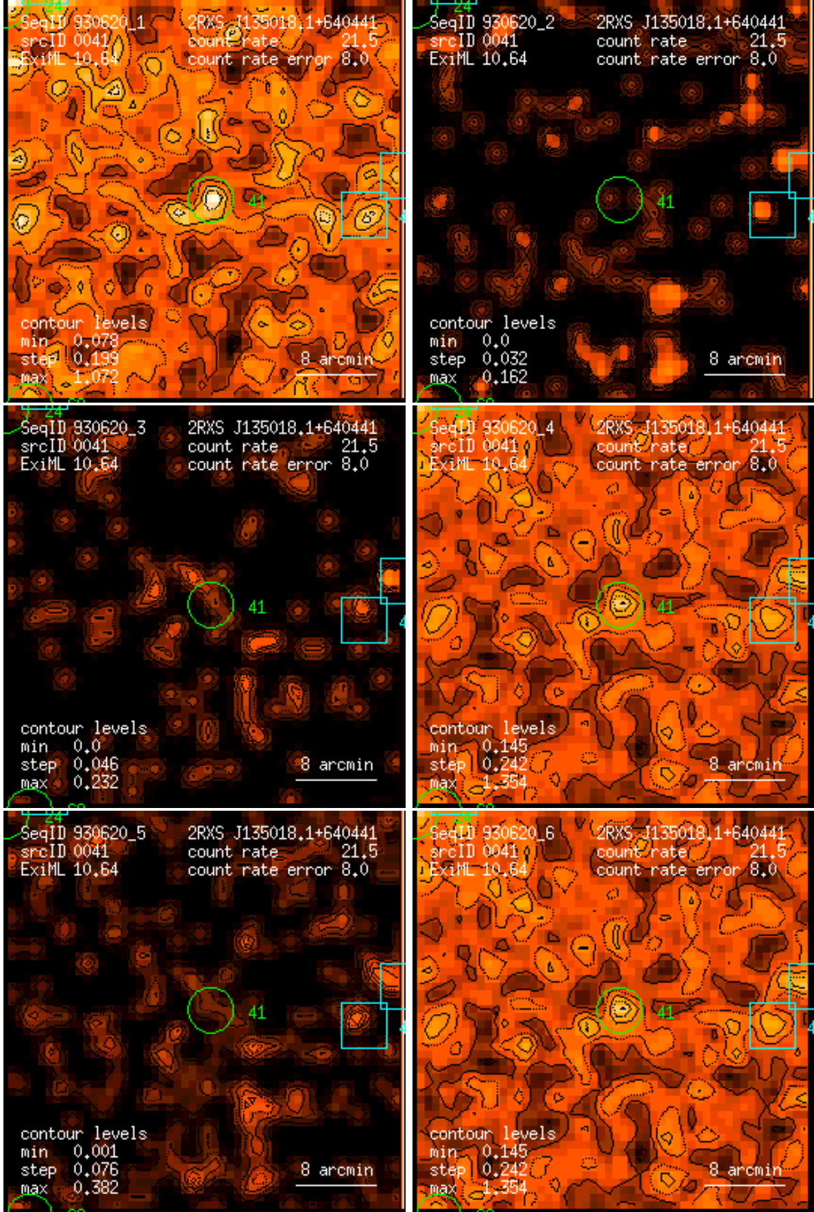
Figure 41: RASS 930620: detection 0041: band rate images, Gaussian filter: (1) PSPC channels 11 – 41, (2) 52 – 90, (3) 91 – 201, (4) 11 – 235, (5) 52 – 201, (6) 11 – 201. Broad band rates in counts/ks. Band rate contour levels in counts/ks/arcmin 2 .
