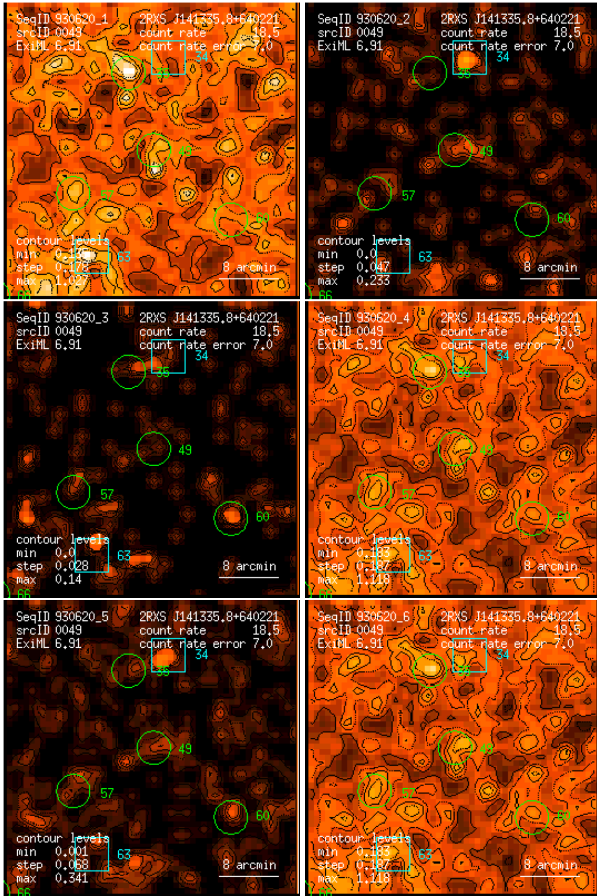
Figure 49: RASS 930620: detection 0049: band rate images, Gaussian filter: (1) PSPC channels 11 – 41, (2) 52 – 90, (3) 91 – 201, (4) 11 – 235, (5) 52 – 201, (6) 11 – 201. Broad band rates in counts/ks. Band rate contour levels in counts/ks/arcmin 2 .
