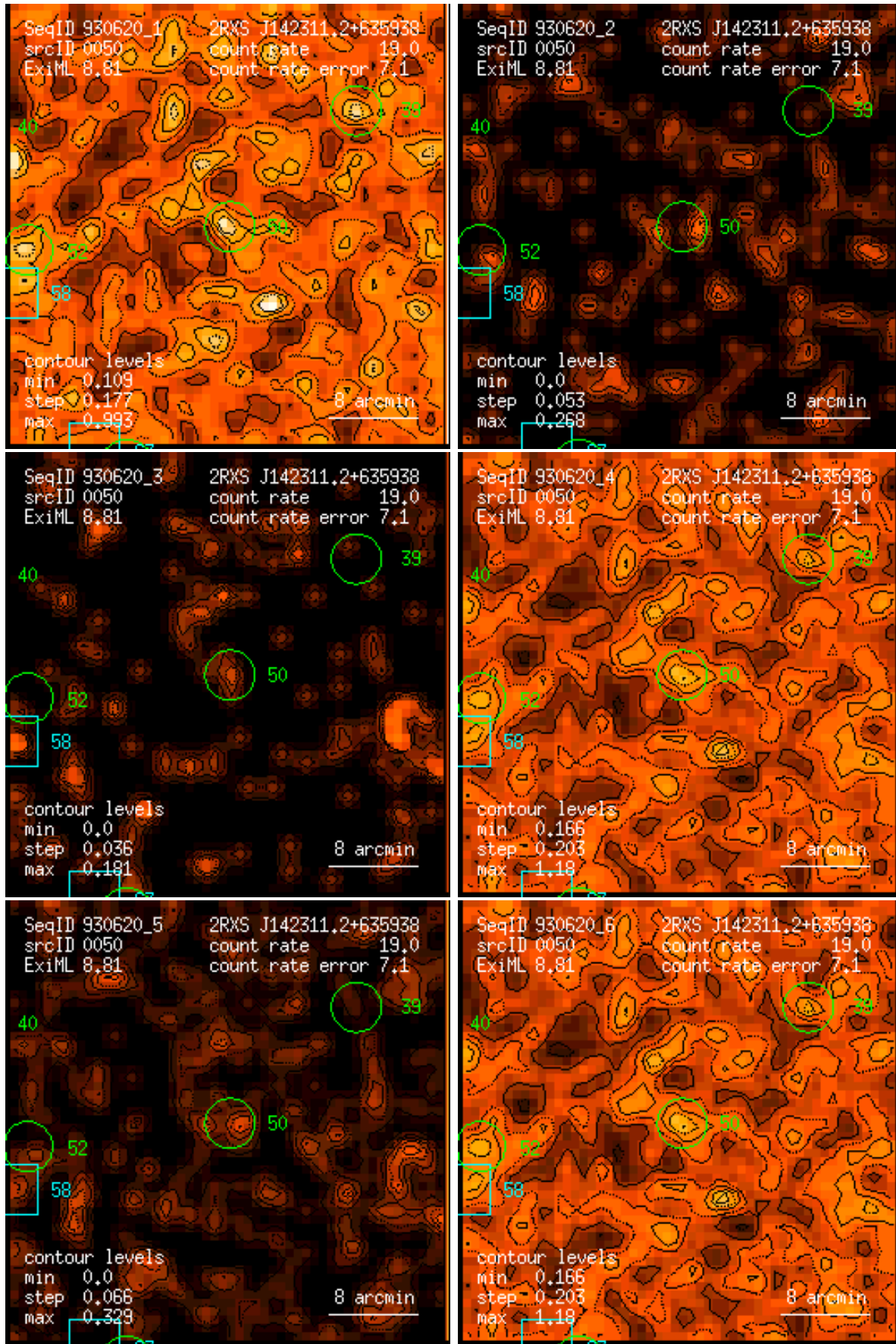
Figure 50: RASS 930620: detection 0050: band rate images, Gaussian filter: (1) PSPC channels 11 – 41, (2) 52 – 90, (3) 91 – 201, (4) 11 – 235, (5) 52 – 201, (6) 11 – 201. Broad band rates in counts/ks. Band rate contour levels in counts/ks/arcmin 2 .
