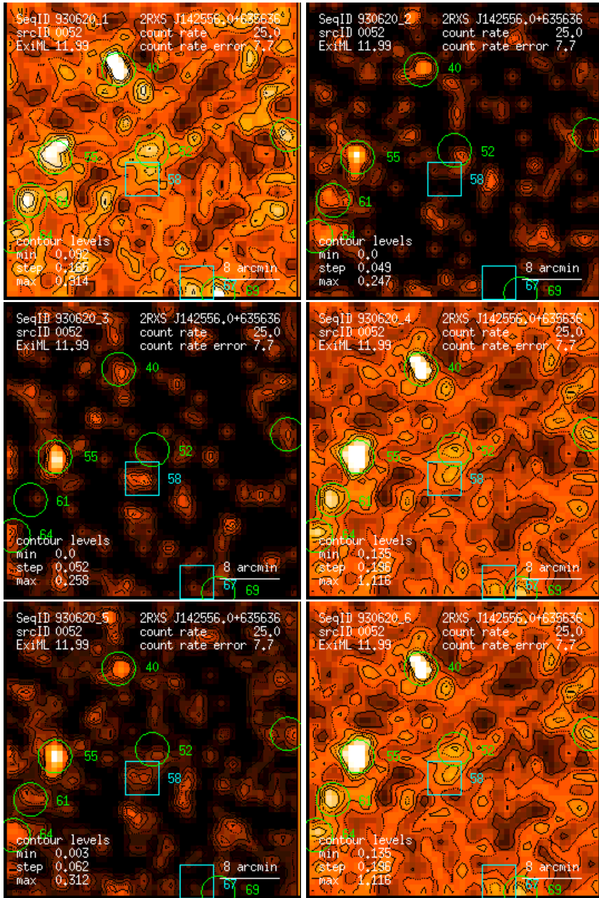
Figure 52: RASS 930620: detection 0052: band rate images, Gaussian filter: (1) PSPC channels 11 – 41, (2) 52 – 90, (3) 91 – 201, (4) 11 – 235, (5) 52 – 201, (6) 11 – 201. Broad band rates in counts/ks. Band rate contour levels in counts/ks/arcmin 2 .
