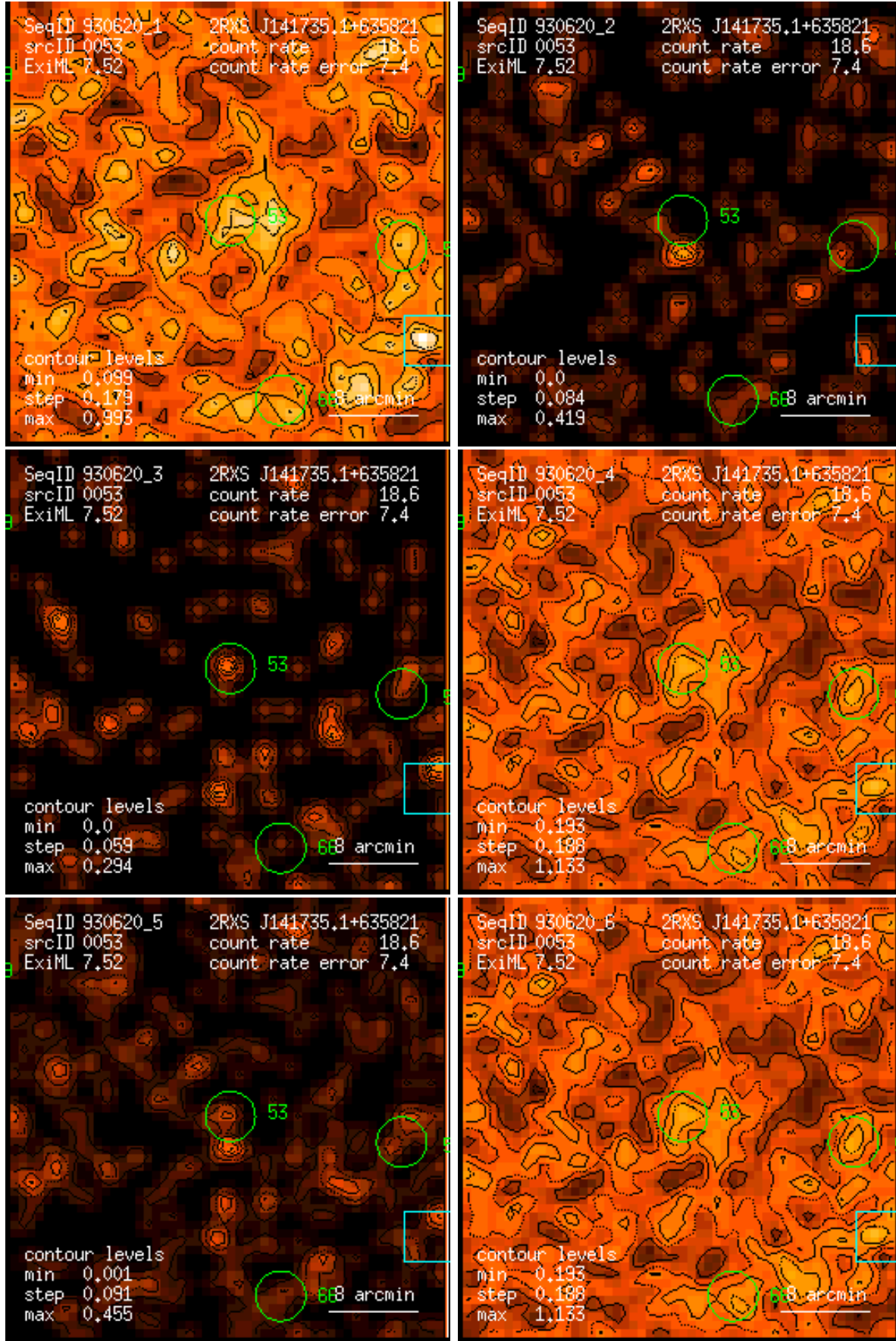
Figure 53: RASS 930620: detection 0053: band rate images, Gaussian filter: (1) PSPC channels 11 – 41, (2) 52 – 90, (3) 91 – 201, (4) 11 – 235, (5) 52 – 201, (6) 11 – 201. Broad band rates in counts/ks. Band rate contour levels in counts/ks/arcmin 2 .
