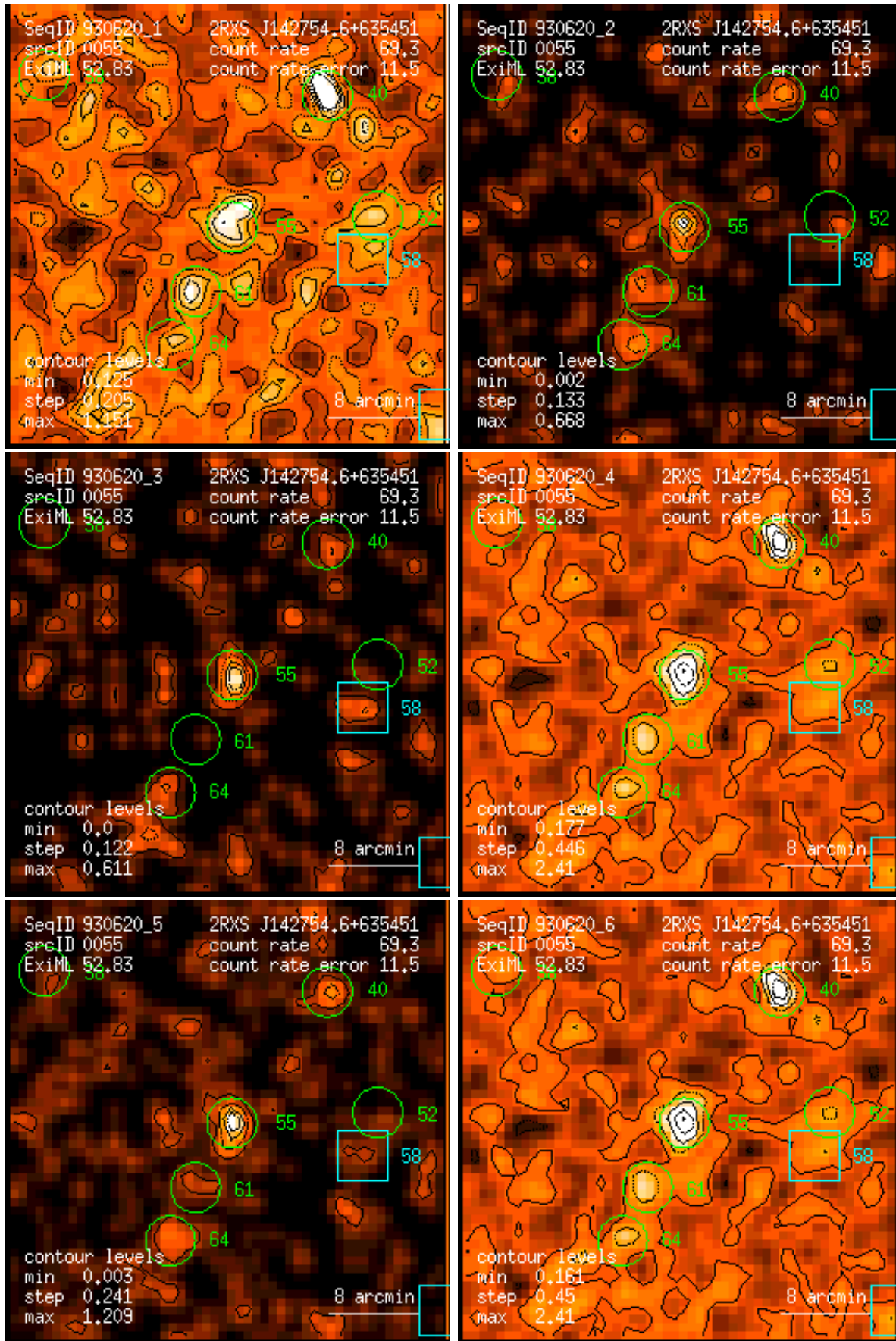
Figure 55: RASS 930620: detection 0055: band rate images, Gaussian filter: (1) PSPC channels 11 – 41, (2) 52 – 90, (3) 91 – 201, (4) 11 – 235, (5) 52 – 201, (6) 11 – 201. Broad band rates in counts/ks. Band rate contour levels in counts/ks/arcmin 2 .
