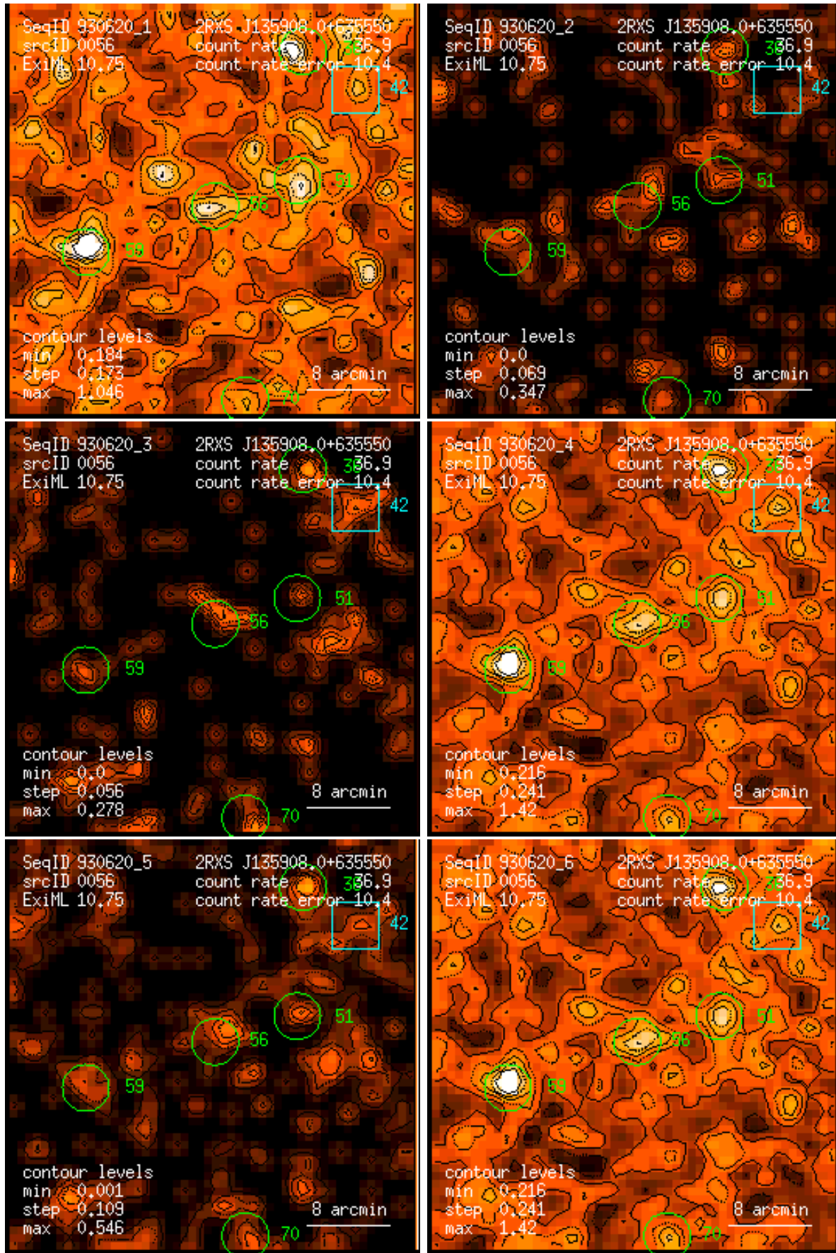
Figure 56: RASS 930620: detection 0056: band rate images, Gaussian filter: (1) PSPC channels 11 – 41, (2) 52 – 90, (3) 91 – 201, (4) 11 – 235, (5) 52 – 201, (6) 11 – 201. Broad band rates in counts/ks. Band rate contour levels in counts/ks/arcmin 2 .
