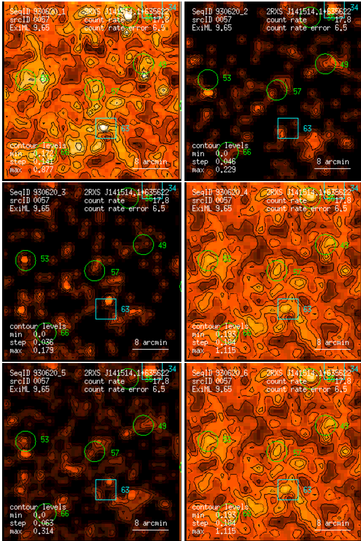
Figure 57: RASS 930620: detection 0057: band rate images, Gaussian filter: (1) PSPC channels 11 – 41, (2) 52 – 90, (3) 91 – 201, (4) 11 – 235, (5) 52 – 201, (6) 11 – 201. Broad band rates in counts/ks. Band rate contour levels in counts/ks/arcmin 2 .
