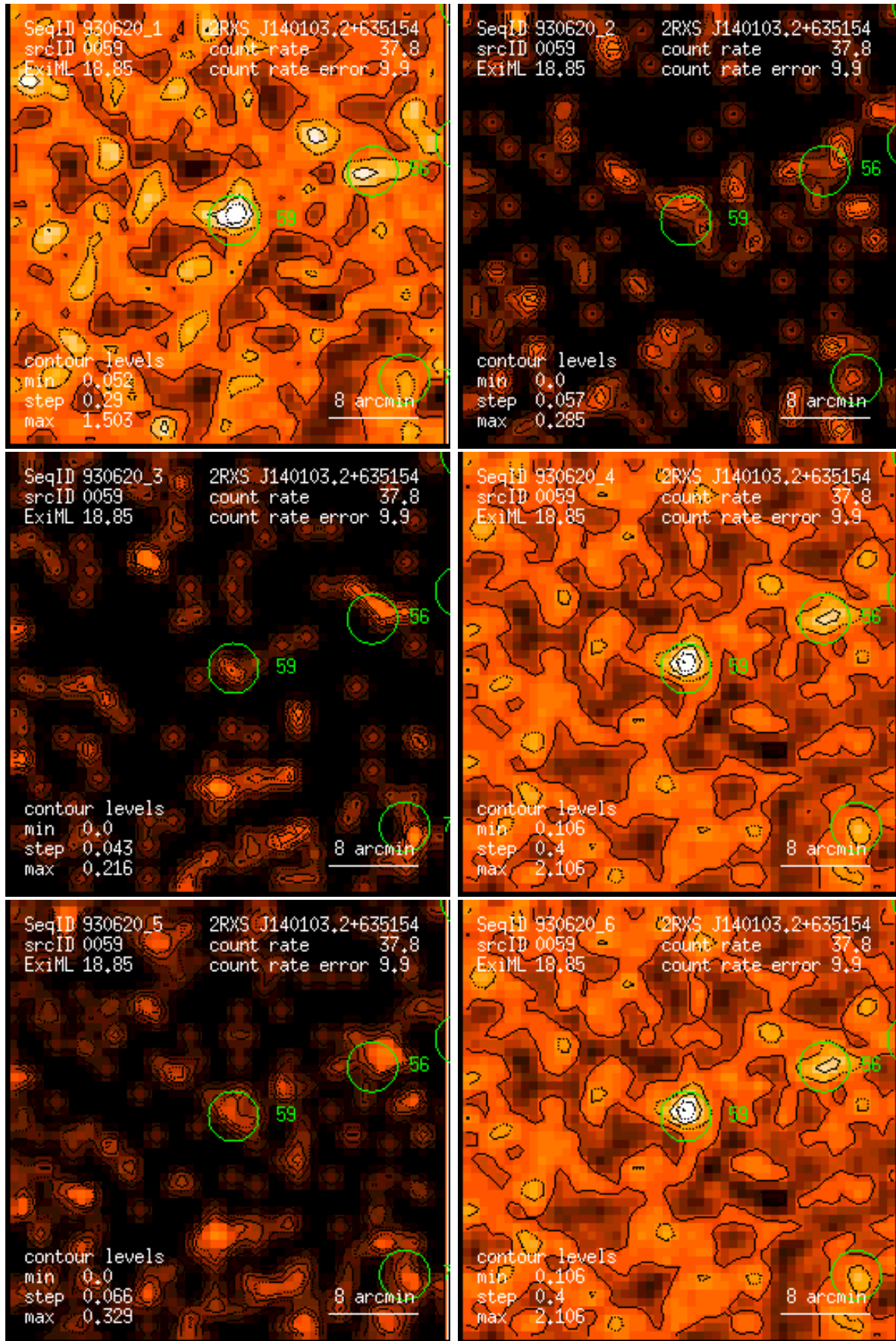
Figure 59: RASS 930620: detection 0059: band rate images, Gaussian filter: (1) PSPC channels 11 – 41, (2) 52 – 90, (3) 91 – 201, (4) 11 – 235, (5) 52 – 201, (6) 11 – 201. Broad band rates in counts/ks. Band rate contour levels in counts/ks/arcmin 2 .
