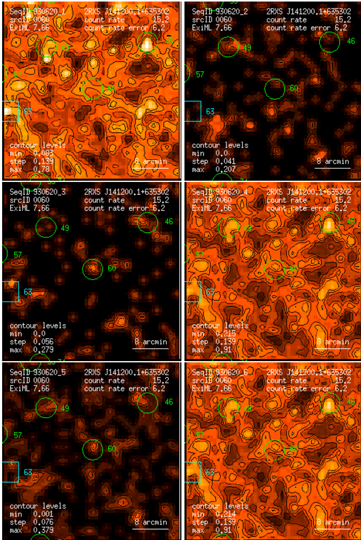
Figure 60: RASS 930620: detection 0060: band rate images, Gaussian filter: (1) PSPC channels 11 – 41, (2) 52 – 90, (3) 91 – 201, (4) 11 – 235, (5) 52 – 201, (6) 11 – 201. Broad band rates in counts/ks. Band rate contour levels in counts/ks/arcmin 2 .
