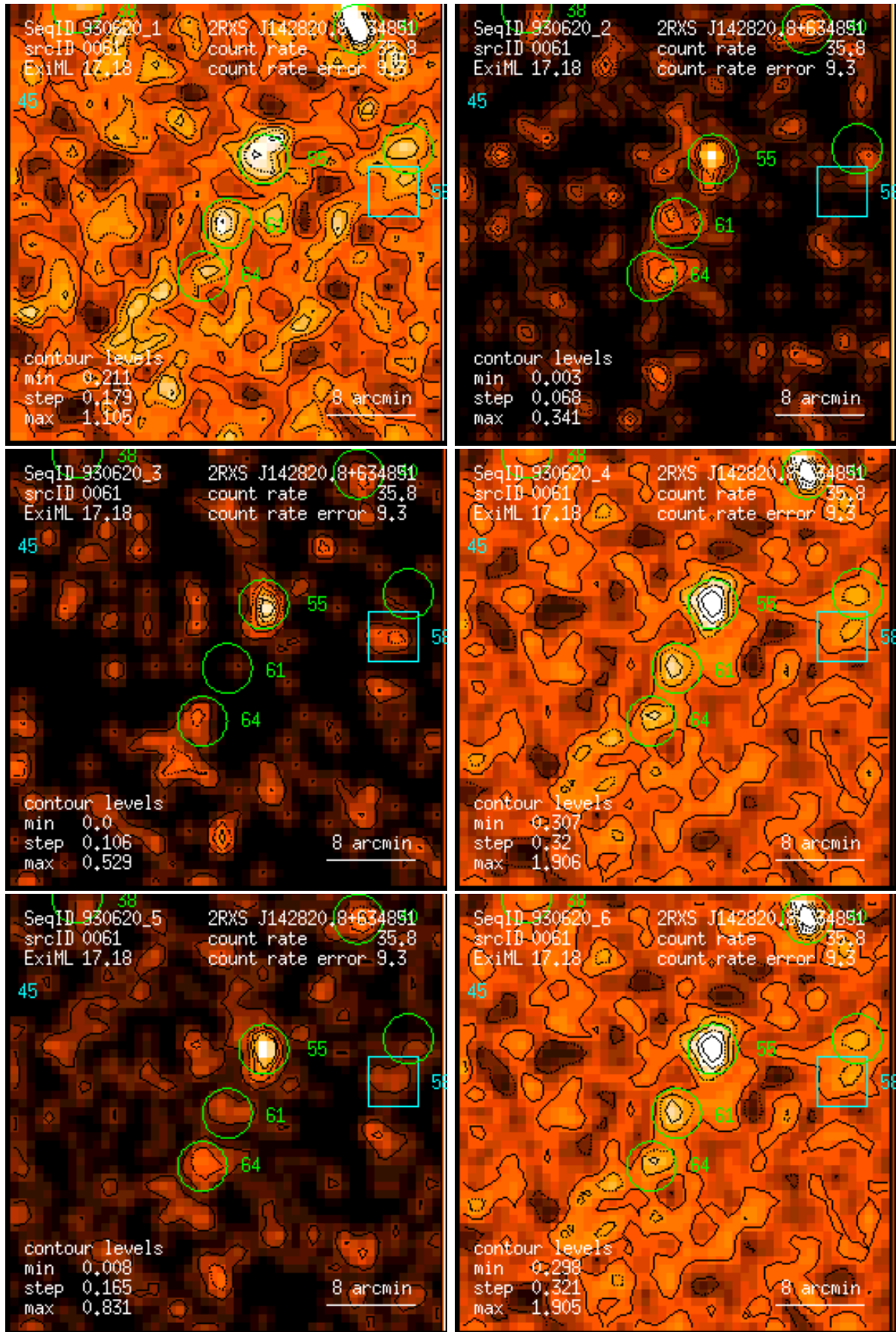
Figure 61: RASS 930620: detection 0061: band rate images, Gaussian filter: (1) PSPC channels 11 – 41, (2) 52 – 90, (3) 91 – 201, (4) 11 – 235, (5) 52 – 201, (6) 11 – 201. Broad band rates in counts/ks. Band rate contour levels in counts/ks/arcmin 2 .
