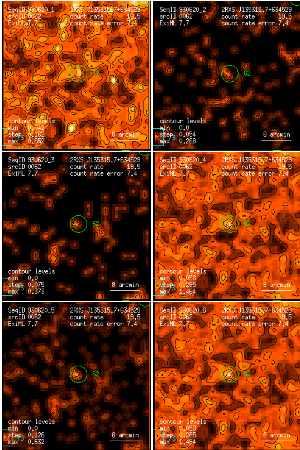
Figure 62: RASS 930620: detection 0062: band rate images, Gaussian filter: (1) PSPC channels 11 – 41, (2) 52 – 90, (3) 91 – 201, (4) 11 – 235, (5) 52 – 201, (6) 11 – 201. Broad band rates in counts/ks. Band rate contour levels in counts/ks/arcmin 2 .
