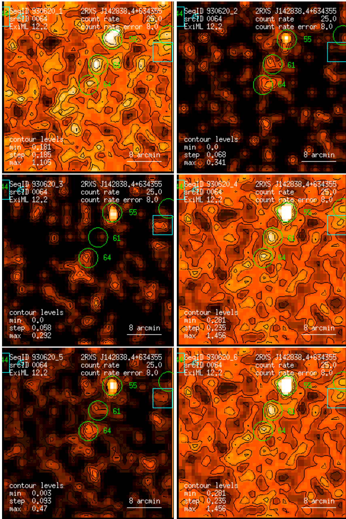
Figure 64: RASS 930620: detection 0064: band rate images, Gaussian filter: (1) PSPC channels 11 – 41, (2) 52 – 90, (3) 91 – 201, (4) 11 – 235, (5) 52 – 201, (6) 11 – 201. Broad band rates in counts/ks. Band rate contour levels in counts/ks/arcmin 2 .
