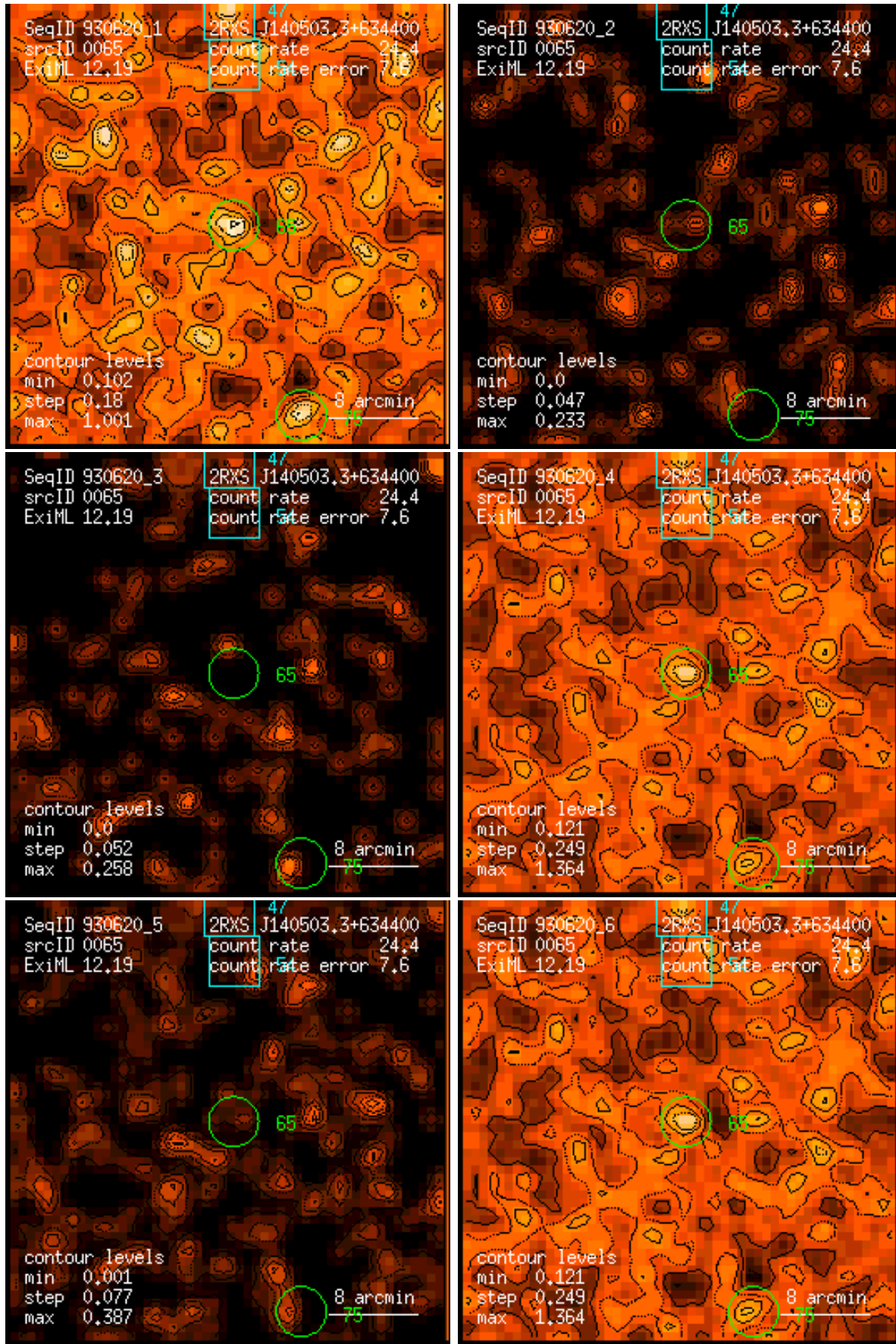
Figure 65: RASS 930620: detection 0065: band rate images, Gaussian filter: (1) PSPC channels 11 – 41, (2) 52 – 90, (3) 91 – 201, (4) 11 – 235, (5) 52 – 201, (6) 11 – 201. Broad band rates in counts/ks. Band rate contour levels in counts/ks/arcmin 2 .
