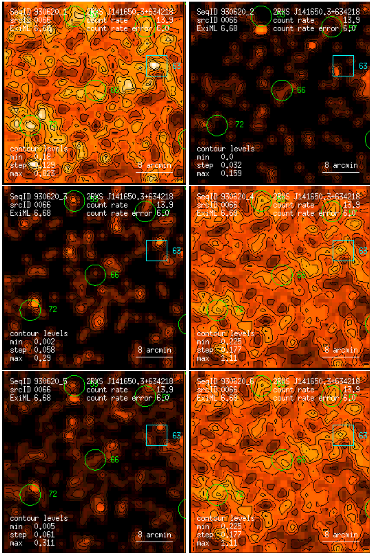
Figure 66: RASS 930620: detection 0066: band rate images, Gaussian filter: (1) PSPC channels 11 – 41, (2) 52 – 90, (3) 91 – 201, (4) 11 – 235, (5) 52 – 201, (6) 11 – 201. Broad band rates in counts/ks. Band rate contour levels in counts/ks/arcmin 2 .
