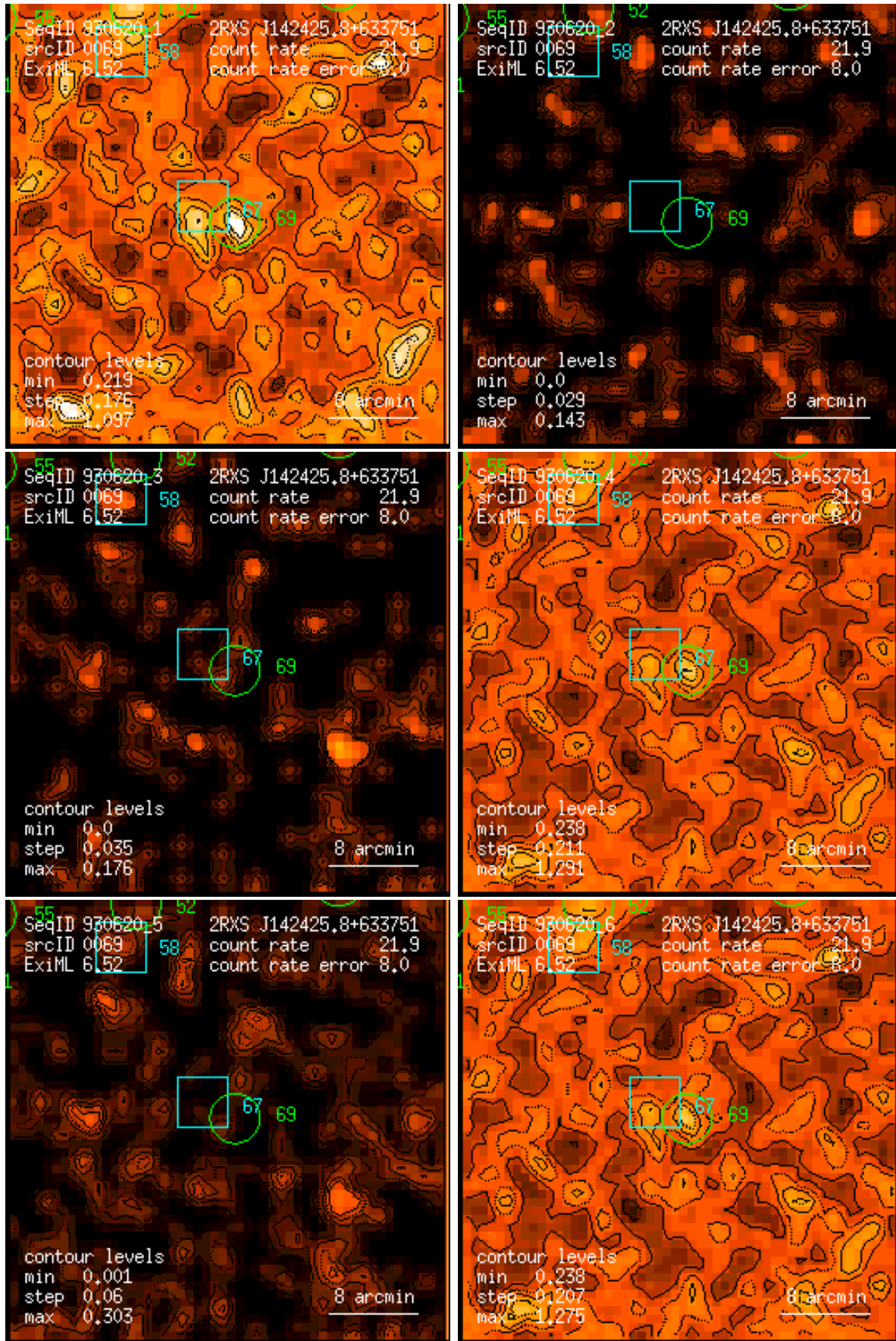
Figure 69: RASS 930620: detection 0069: band rate images, Gaussian filter: (1) PSPC channels 11 – 41, (2) 52 – 90, (3) 91 – 201, (4) 11 – 235, (5) 52 – 201, (6) 11 – 201. Broad band rates in counts/ks. Band rate contour levels in counts/ks/arcmin 2 .
