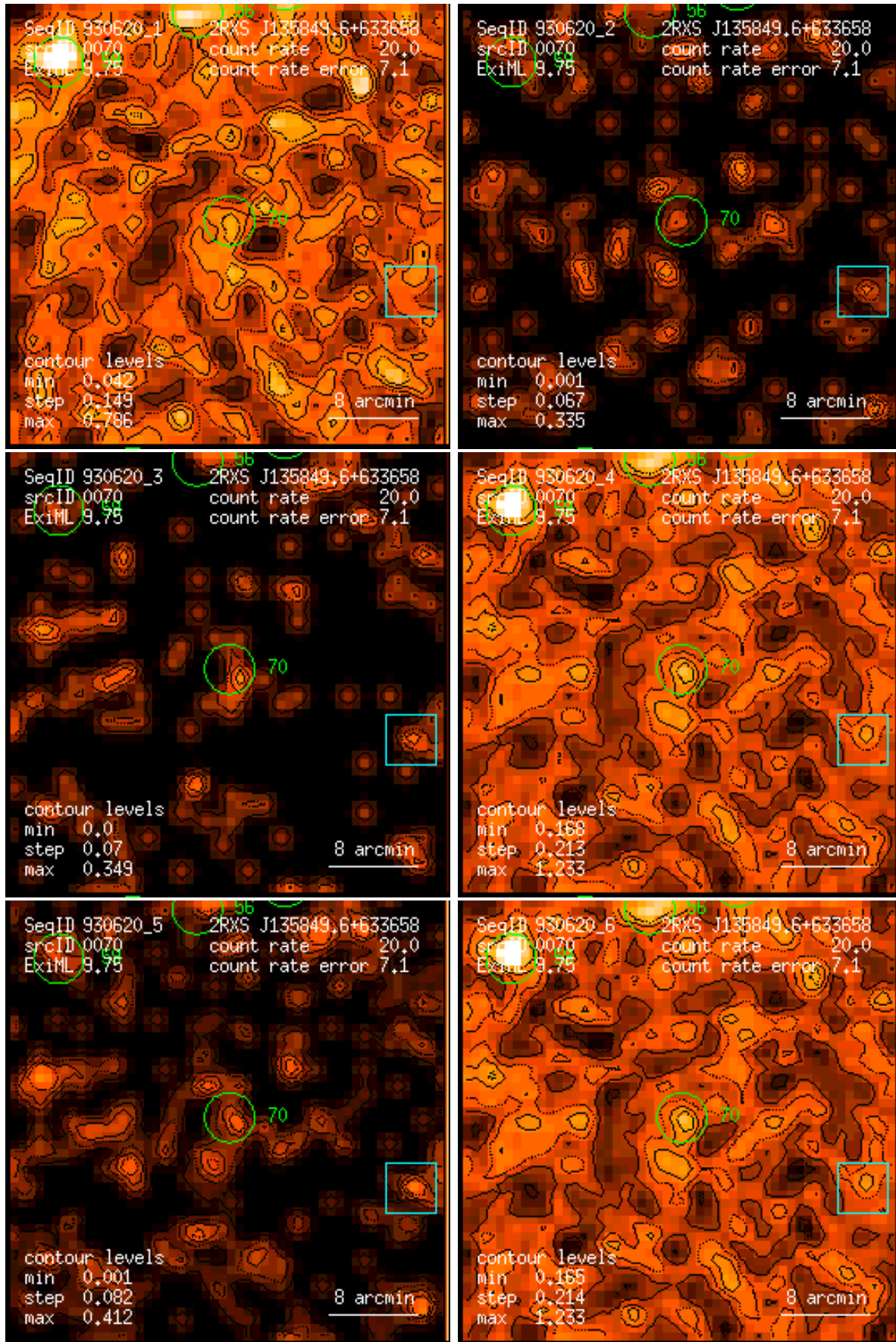
Figure 70: RASS 930620: detection 0070: band rate images, Gaussian filter: (1) PSPC channels 11 – 41, (2) 52 – 90, (3) 91 – 201, (4) 11 – 235, (5) 52 – 201, (6) 11 – 201. Broad band rates in counts/ks. Band rate contour levels in counts/ks/arcmin 2 .
