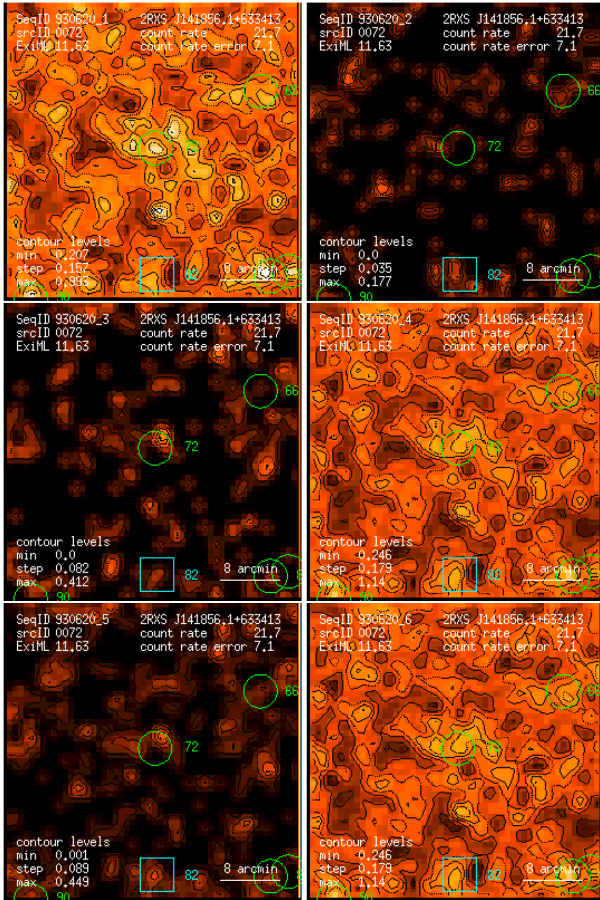
Figure 72: RASS 930620: detection 0072: band rate images, Gaussian filter: (1) PSPC channels 11 – 41, (2) 52 – 90, (3) 91 – 201, (4) 11 – 235, (5) 52 – 201, (6) 11 – 201. Broad band rates in counts/ks. Band rate contour levels in counts/ks/arcmin 2 .
